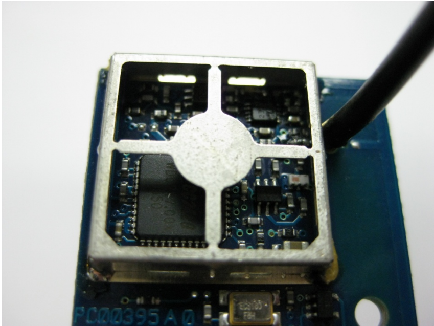
Close Up of RF Section, View #4
