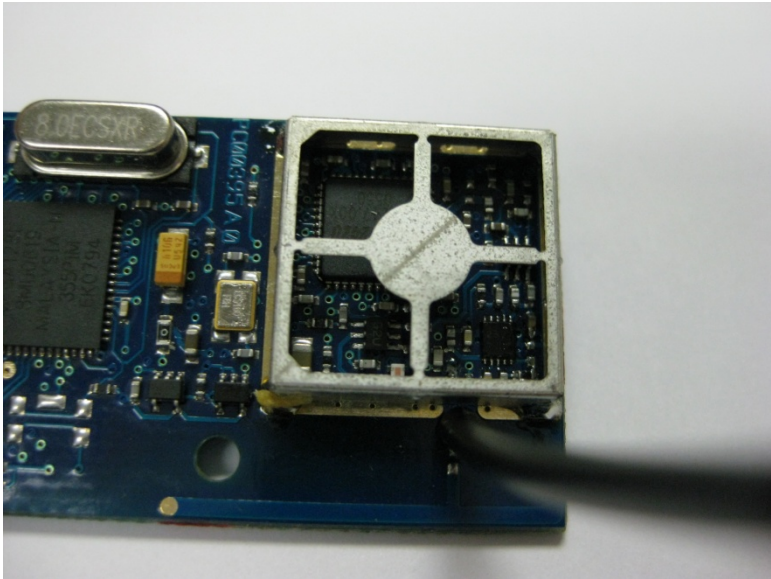
Close Up of RF Section, View #2
