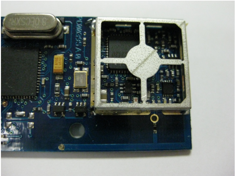
Close Up of RF Section, View #1
