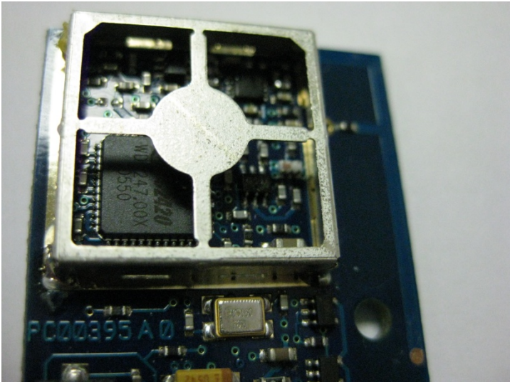
Close Up of RF Section, View #3
