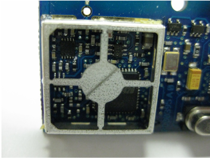
Close Up of RF Section, View #4
