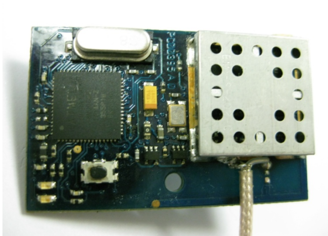
Close Up of Board, Showing Antenna Connection Point
