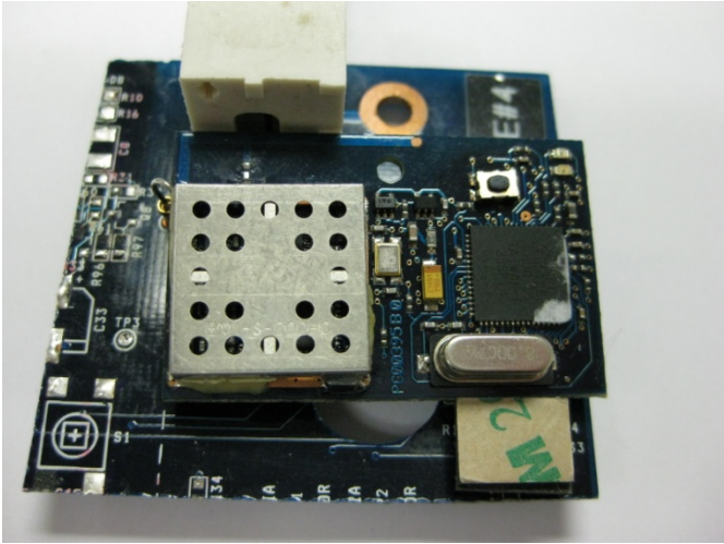
Close Up of Module on Board, View #1
