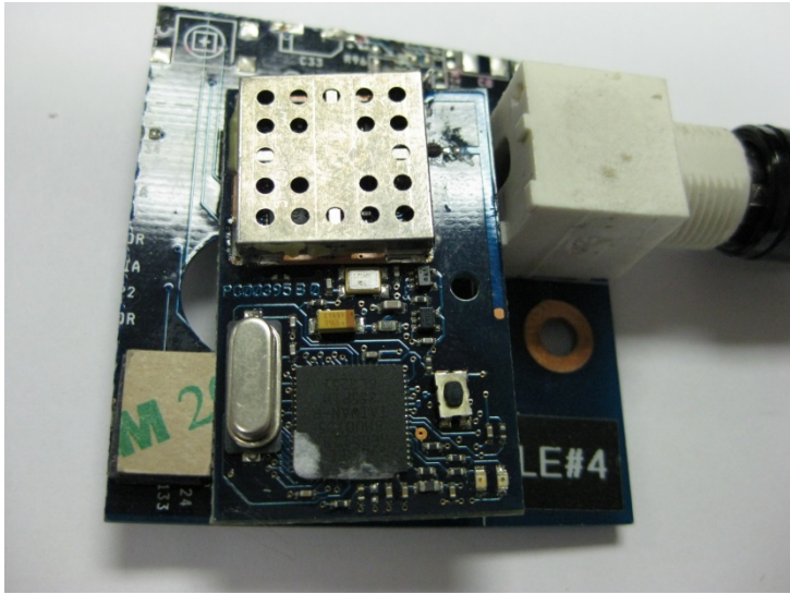
Close Up of Module on Board, View #2
