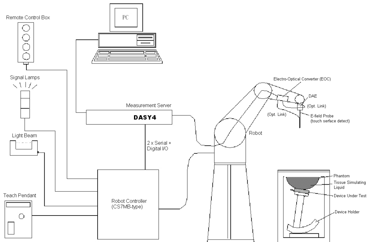
Fig. 5.1 DASY4 System
