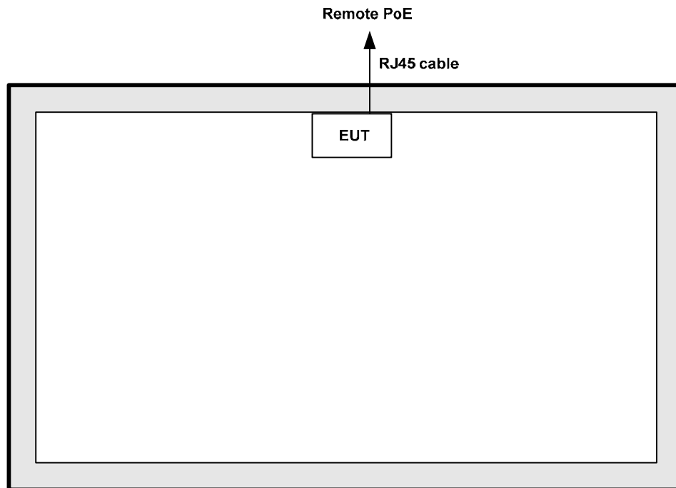
Test Setup Diagram - Radiated Emission mode 1 (Above 1GHz)
