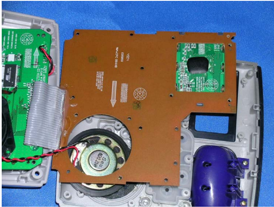
Base TAD and keypad PCB rear side
