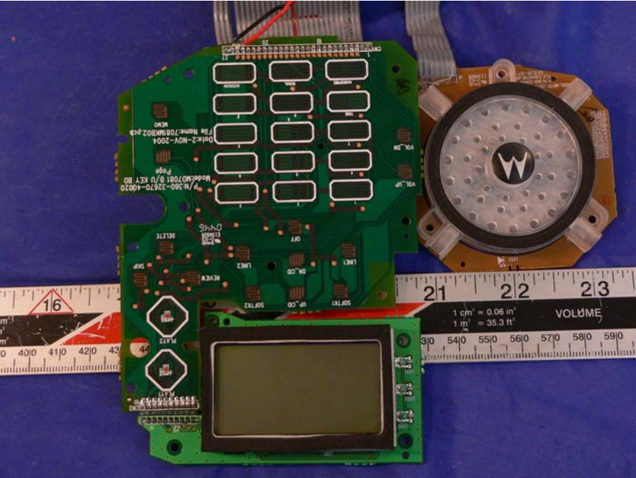
Base- LCD Keypad Board Solder View
