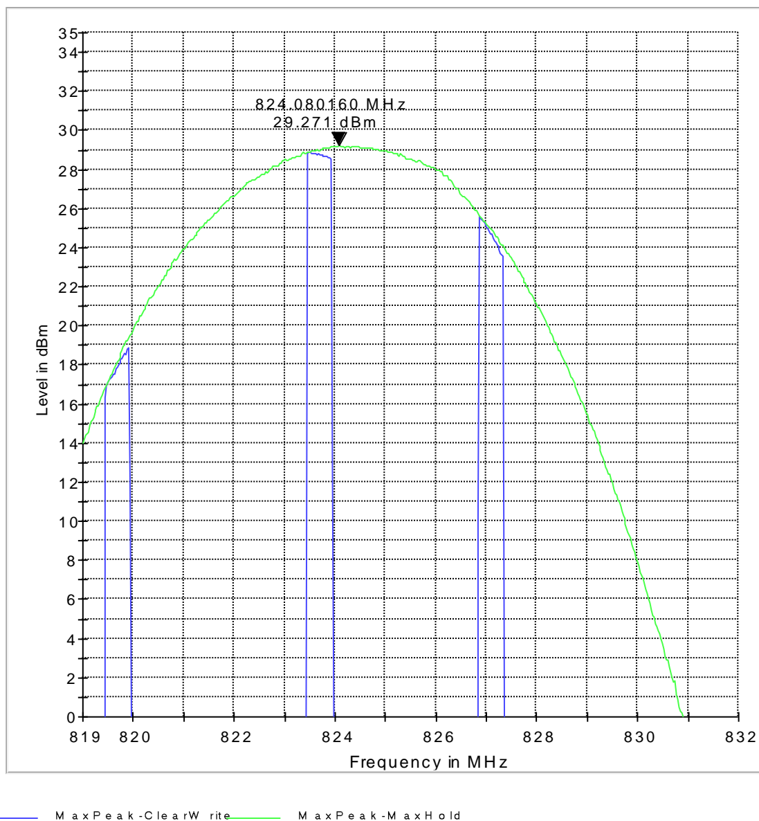
ERP 850 L
