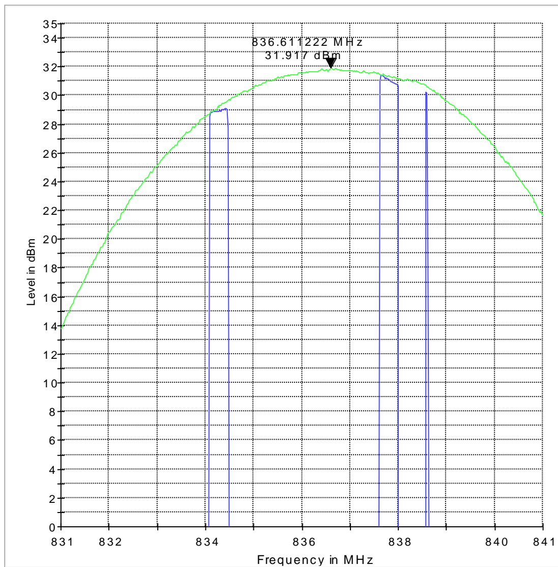
ERP 850 M
