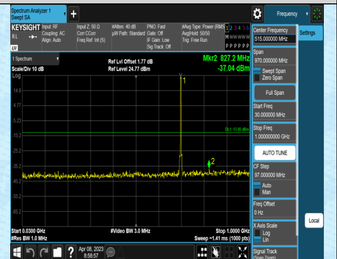
Band12-3MHz-16QAM-23165-1RB#0-Range1:30~1000 MHz
