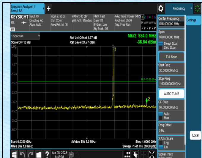
Band12-1.4MHz-16QAM-23095-1RB#0-Range1:30~100 0MHz
