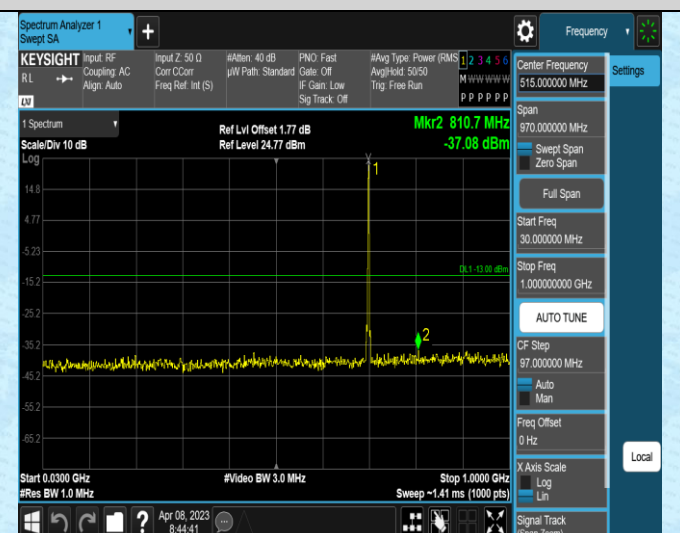
Band12-1.4MHz-16QAM-23173-1RB#0-Range1:30~100 0MHz
