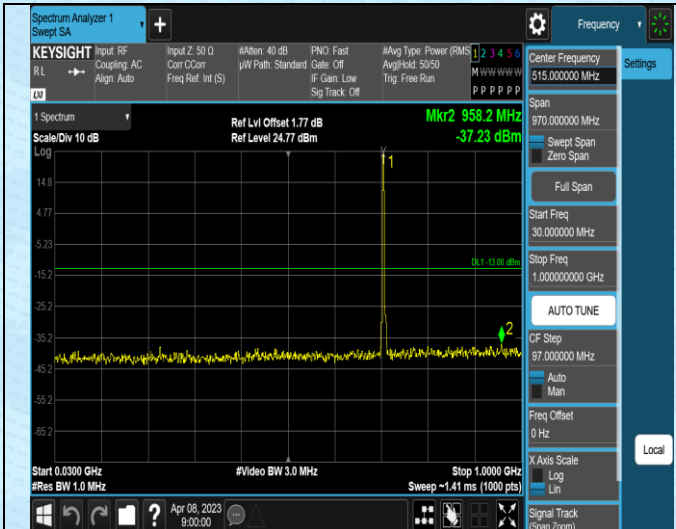
Band12-5MHz-QPSK-23035-1RB#0-Range2:30~1000M
