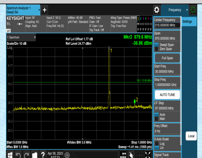
Band12-3MHz-QPSK-23095-1RB#0-Range1:30~1000M
