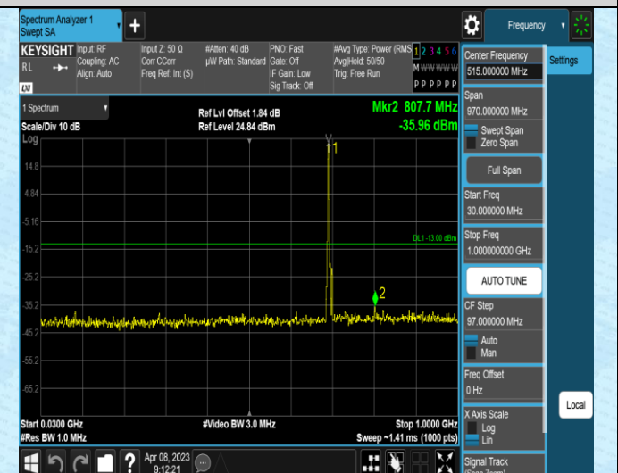
Band12-5MHz-QPSK-23095-1RB#0-Range1:30~1000M
