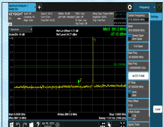
Band12-3MHz-QPSK-23025-1RB#0-Range1:30~1000M
