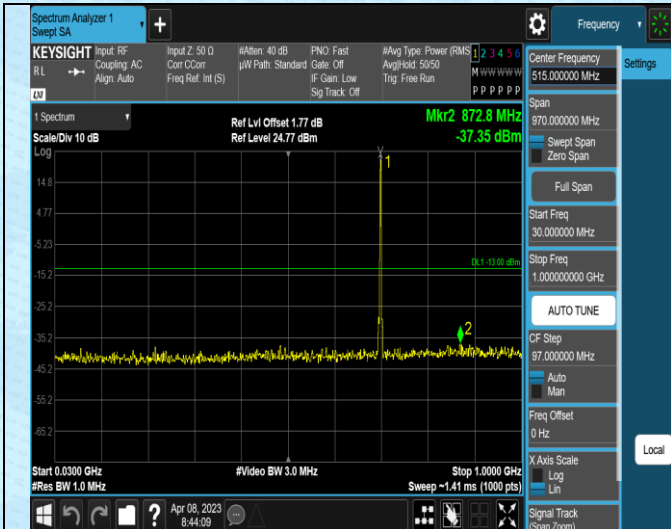
Band12-1.4MHz-QPSK-23173-1RB#0-Range2:30~1000 MHz
