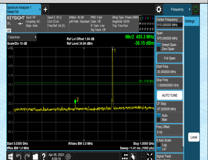
Band12-3MHz-16QAM-23025-1RB#0-Range1:30~1000
