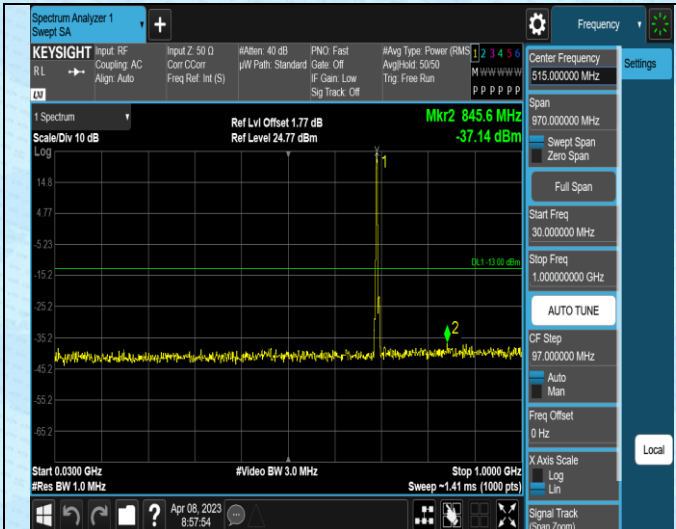
Band12-3MHz-16QAM-23095-1RB#0-Range1:30~1000 MHz
