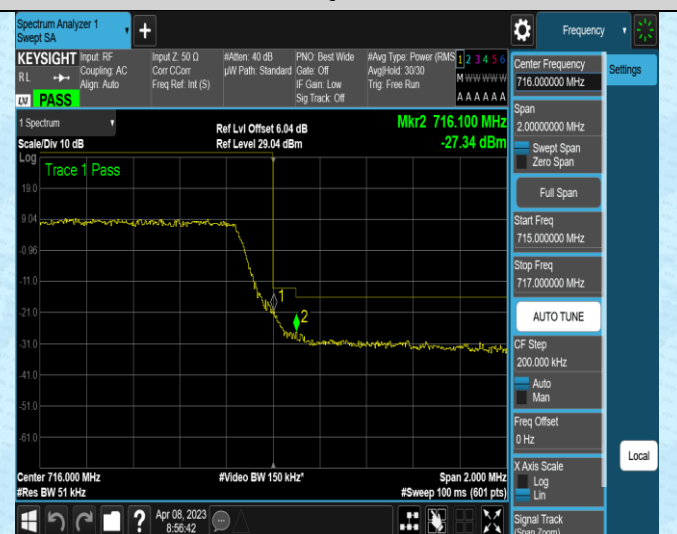
Band12-5MHz-QPSK-23155-25RB#0
