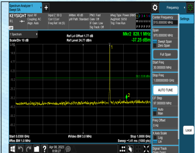
Band12-3MHz-QPSK-23165-1RB#0-Range2:30~1000M
