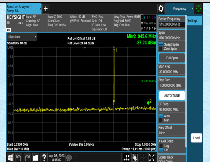
Band12-1.4MHz-16QAM-23017-1RB#0-Range1:30~100 0MHz
