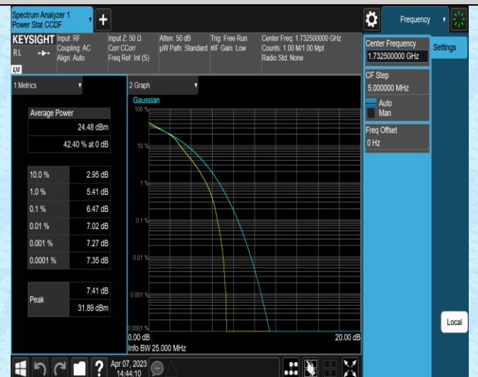
Band4-5MHz-16QAM-20375-25RB#0
