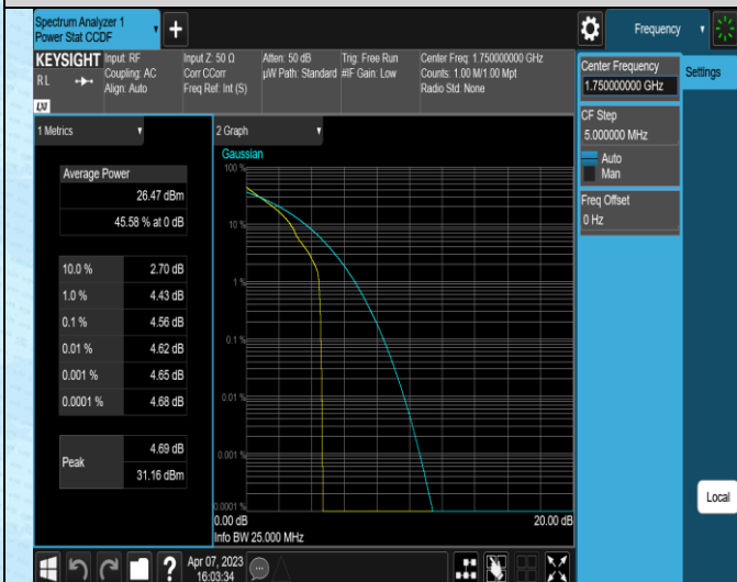
Band4-10MHz-16QAM-20000-1RB#0
