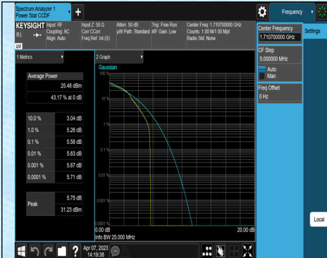
Band4-1.4MHz-16QAM-20175-1RB#0
