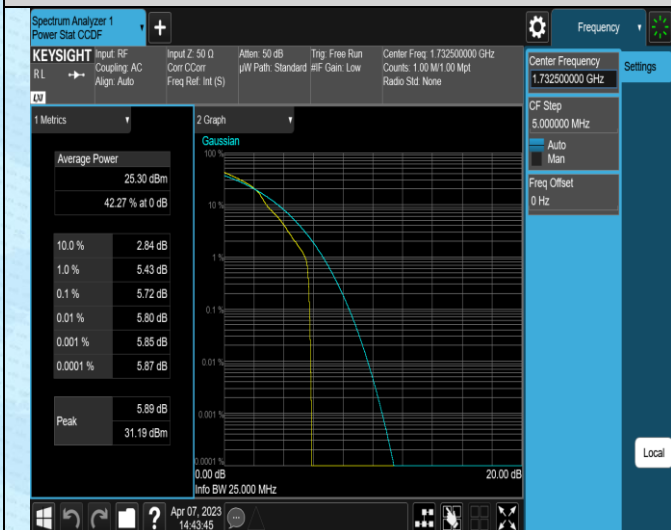
Band4-5MHz-16QAM-20375-1RB#0
