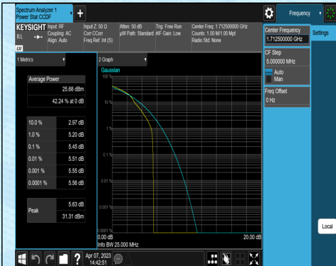
Band4-5MHz-16QAM-20175-1RB#0
