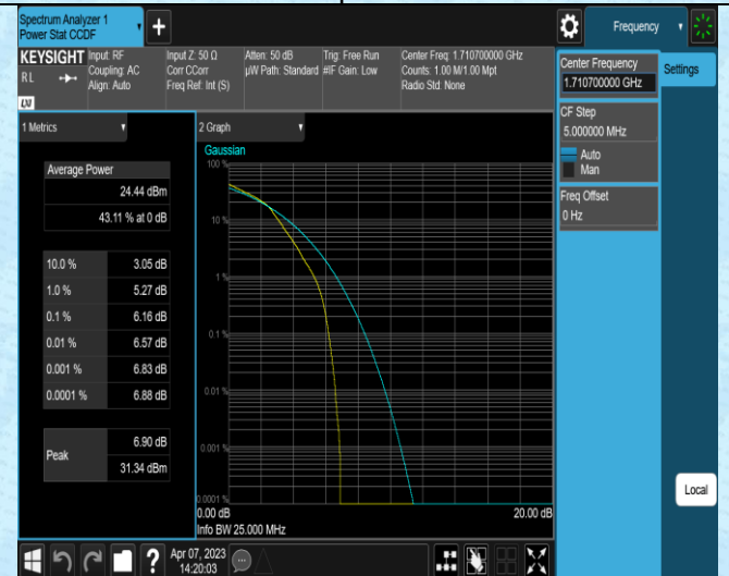
Band4-1.4MHz-16QAM-20175-6RB#0
