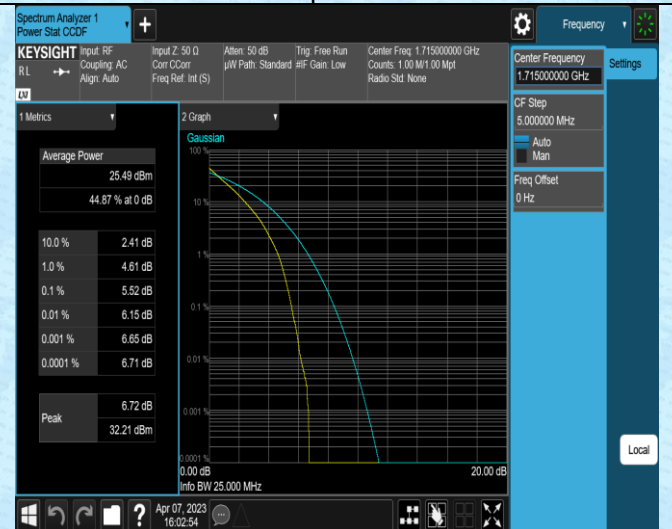
Band4-10MHz-QPSK-20175-50RB#0
