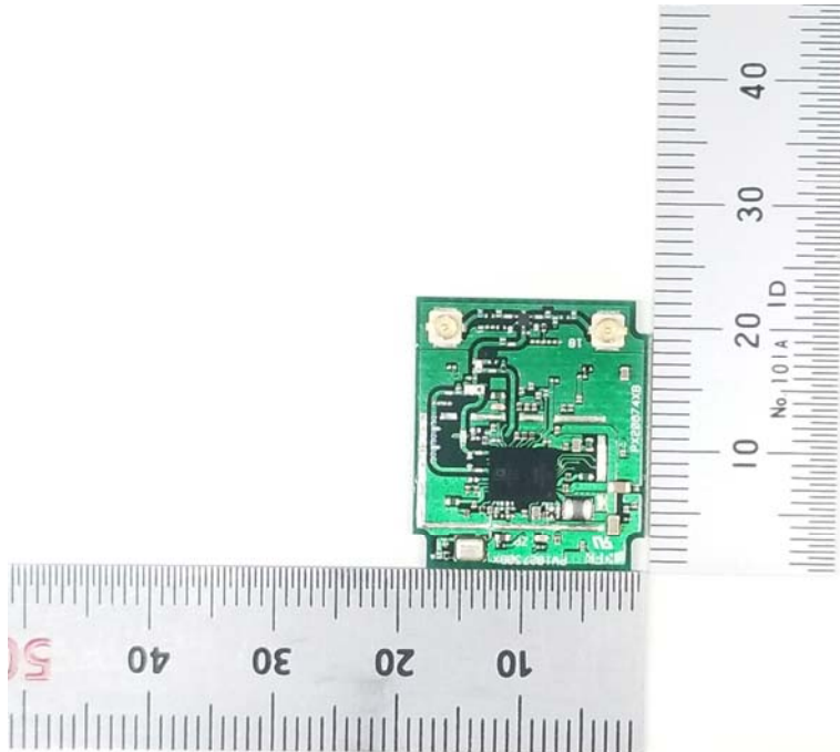
Internal View of EUT
