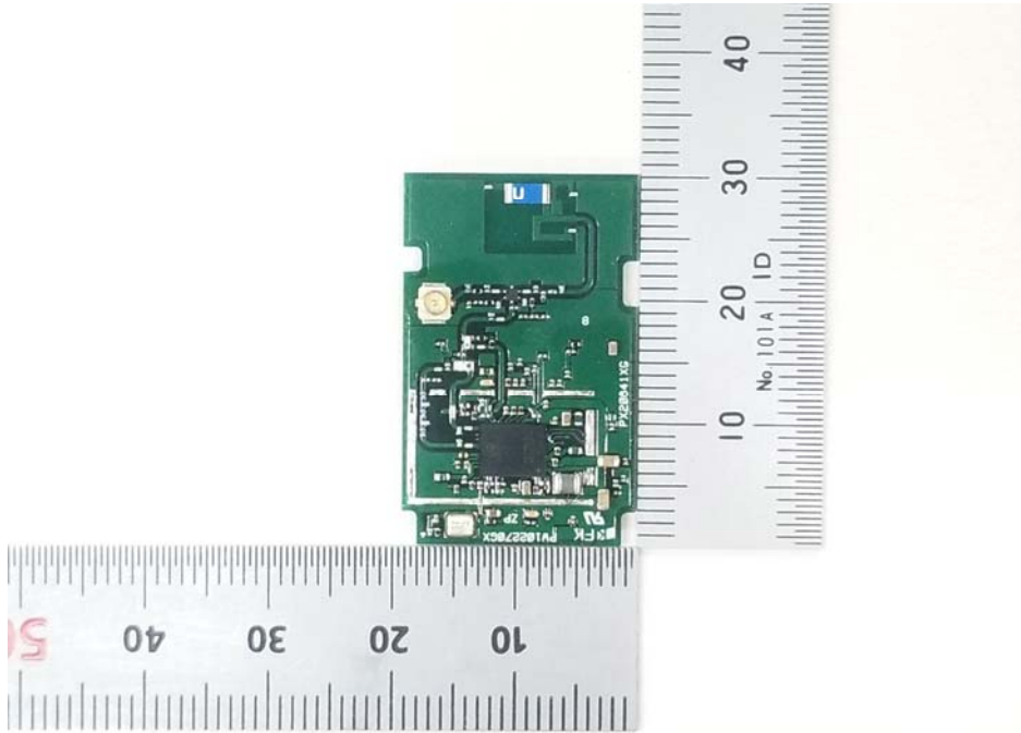
Internal View of EUT
