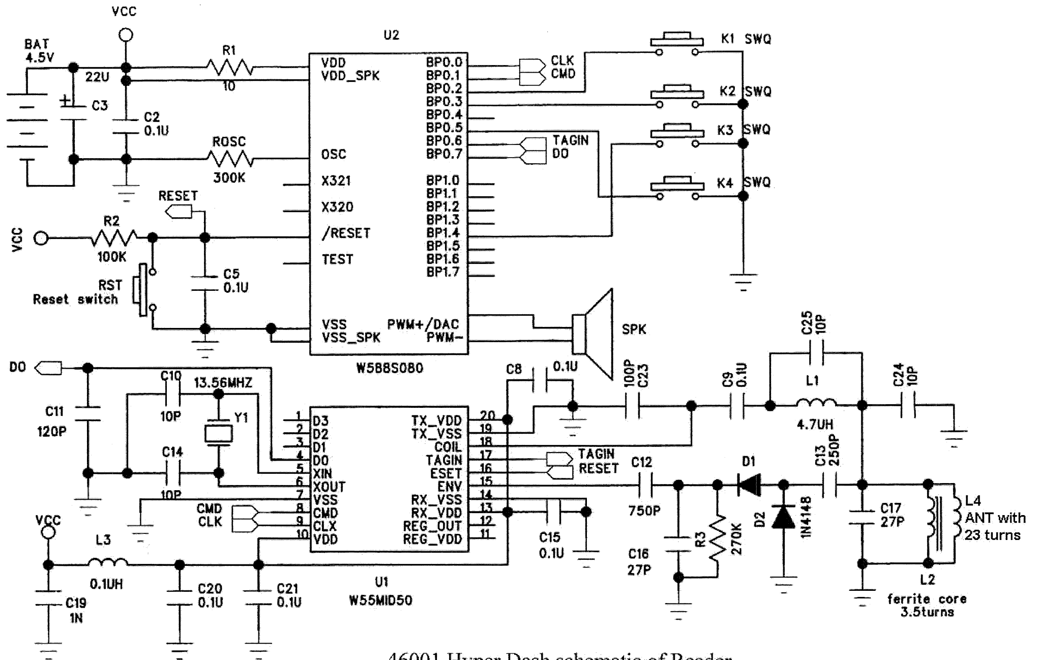
46001 Hyper Dash schematic of Reader
