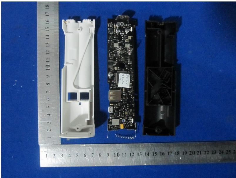
Photo 12 Internal of EUT (Indoor)
