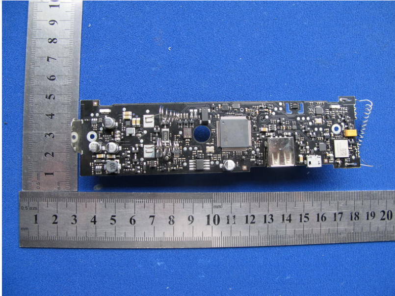
Photo 13 Appearance of PCB (Indoor)
