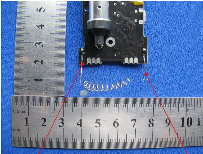
Photo 15 Appearance of Antenna (Indoor)
