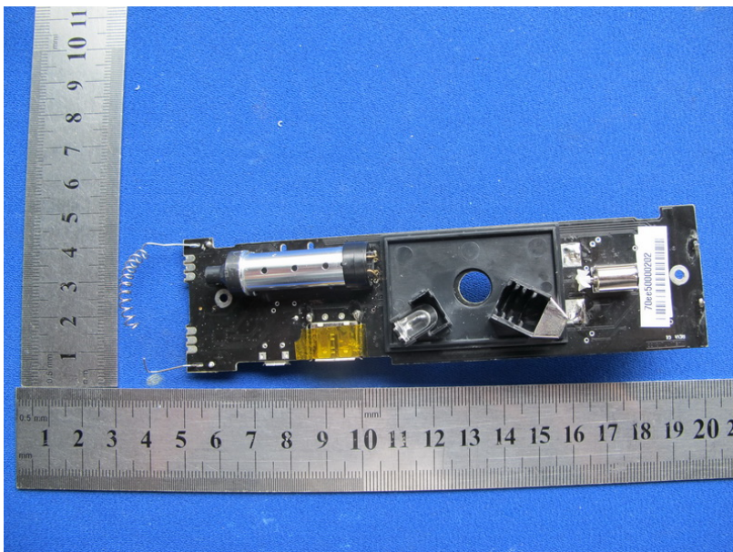
Photo 14 Appearance of PCB (Indoor)
