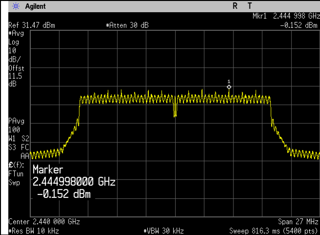
Mid Ch_2440MHz_20MHz_Spectral Density_Port 1
