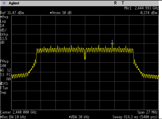
Mid Ch_2440MHz_20MHz_Spectral Density_Port 2
