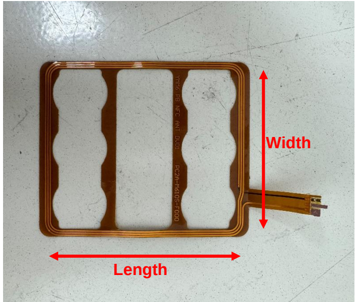
FPCB Antenna(YMM614)
