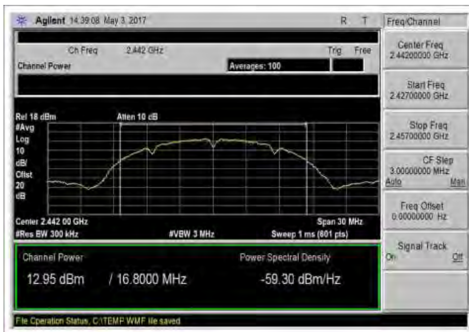
802.11b_Middle Channel_2442MHz_PowerOutput
