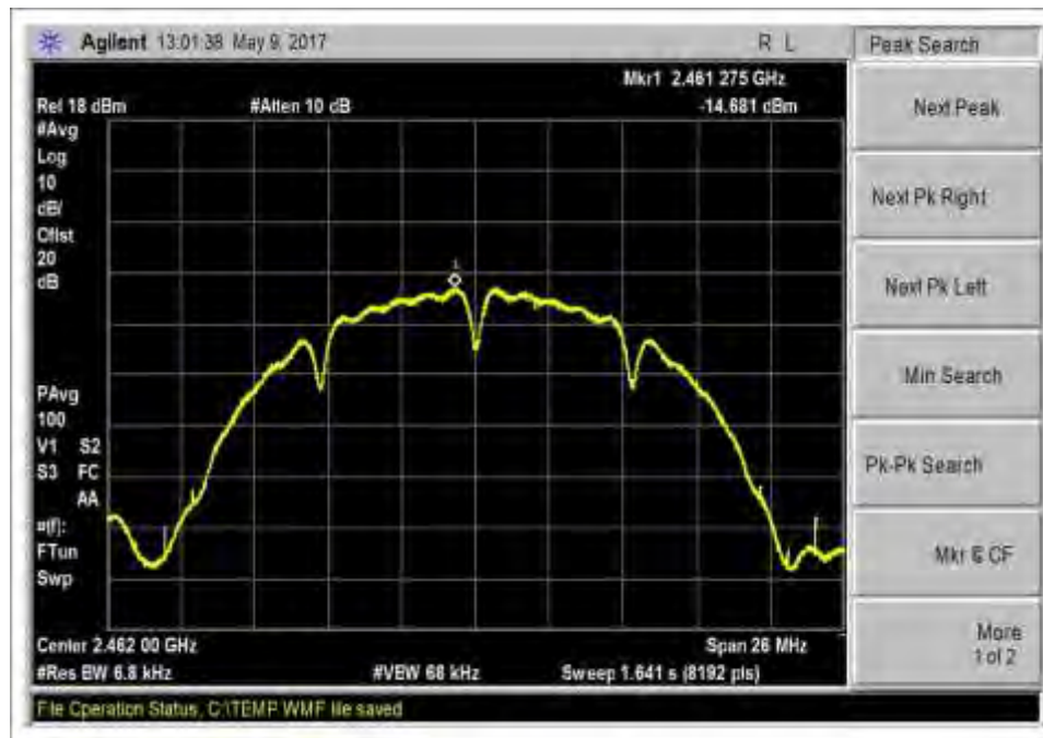
802.11b_High Channel_2462MHz_PSD
