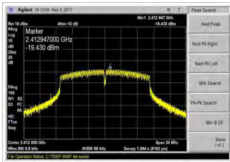
802.11g_Low Channel_2412MHz_PSD
