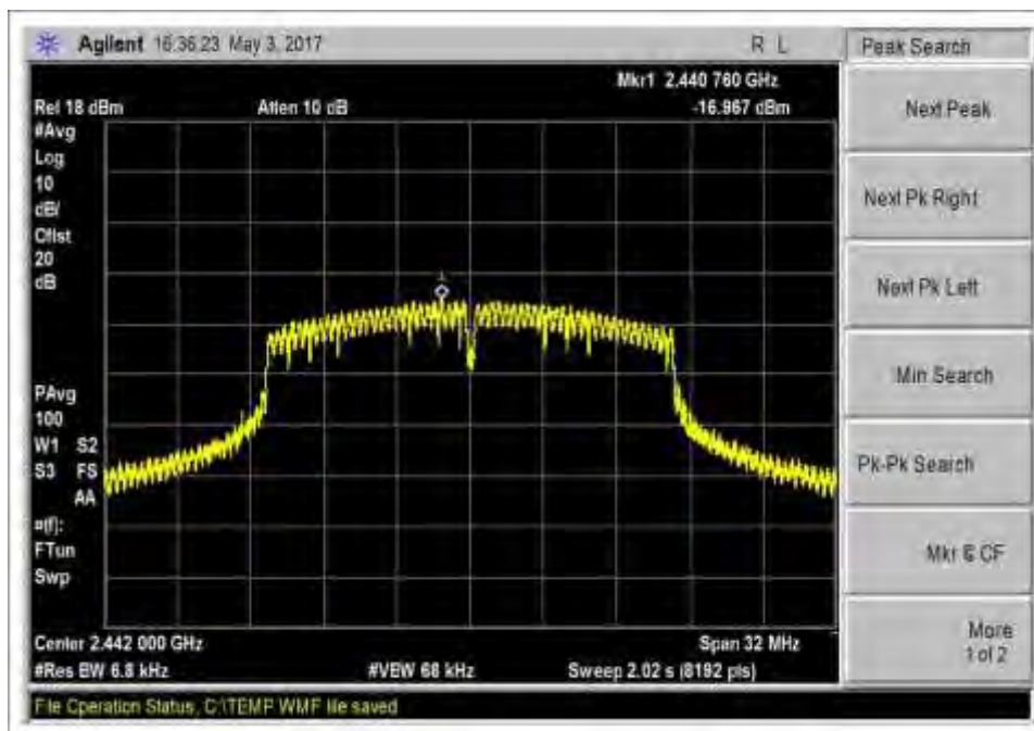
802.11n20_Middle Channel_2442MHz_PSD
