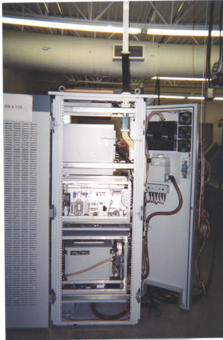
EXTERIOR PHOTOGRAPH FCC IDENTIFIER #MTOTDR3070A-C1 RADTEC ENGINEERING, INC.
