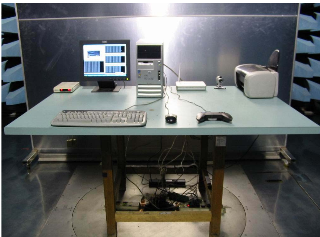
Front View of the Test Configuration
