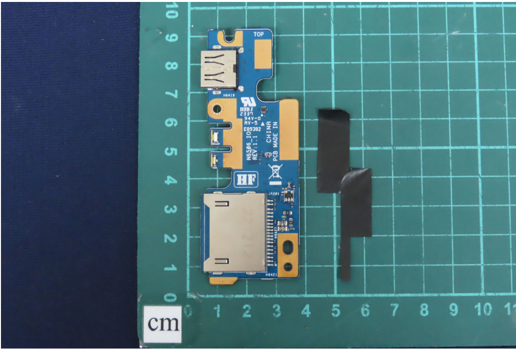
(32) EUT Photo
