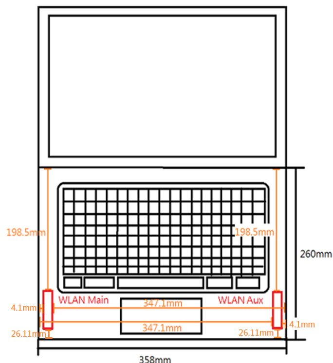
Photograph 17. Antenna position of EUT
