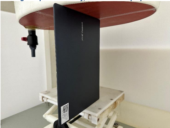
Testing Setup for Extremity, Left Side of Laptop at 0 mm
