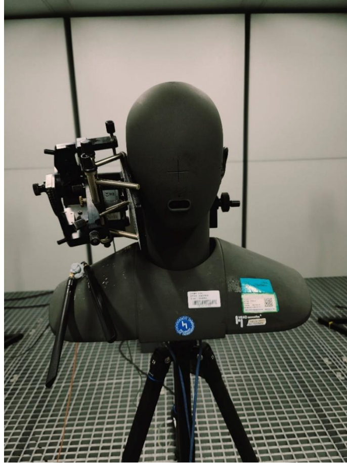
Figure E-1 – Test Layout (Handset)
