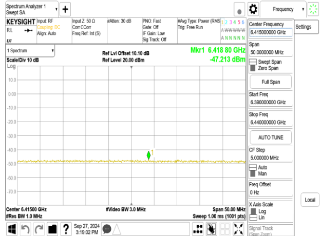
802.11be_20MHz_Chain0_6415MHz_106+26_MRU2
