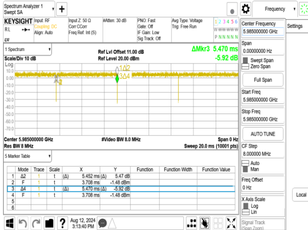
802.11be_80MHz_Chain0_5985MHz_RU484+242_Punc20
