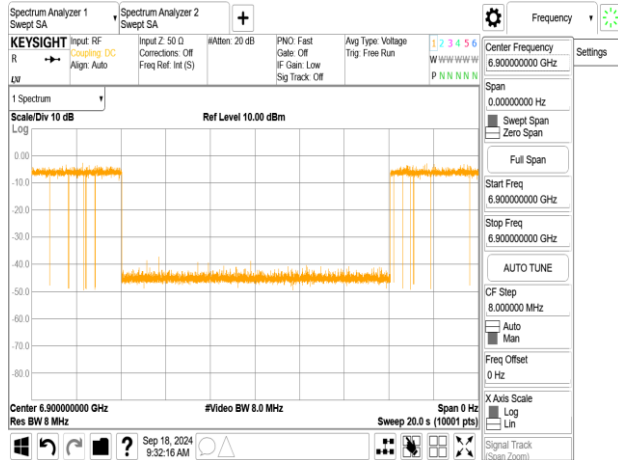
802.11be_320MHz_CF 6745MHz_Interference_6900MHz_-80.26dBm_Minimal
