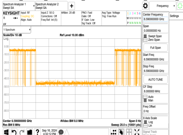
802.11be_320MHz_CF 6745MHz_Interference_6590MHz_-79.05dBm_Minimal
