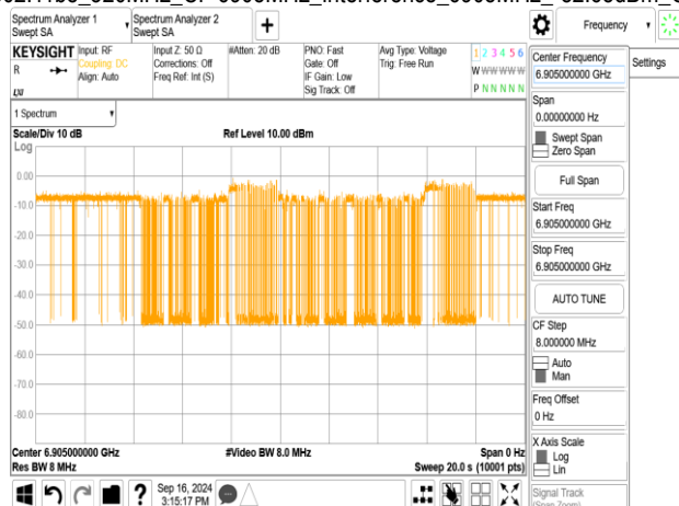
802.11be_320MHz_CF 6905MHz_Interference_6905MHz_-82.65dBm_ON
