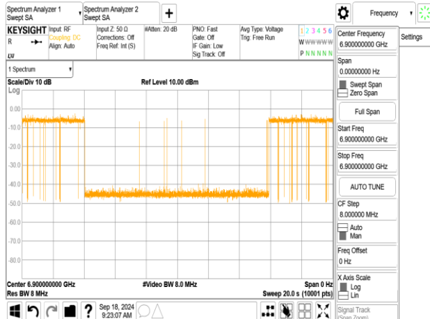
802.11be_320MHz_CF 6745MHz_Interference_6900MHz_-82.26dBm_ON
