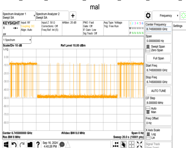
802.11be_320MHz_CF 6745MHz_Interference_6745MHz_-79.25dBm_ON
