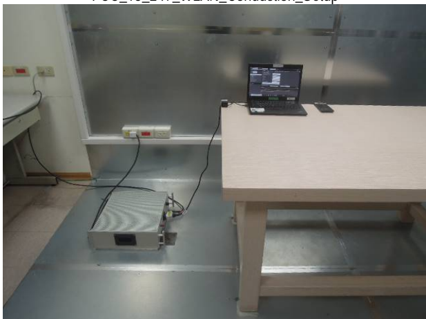
FCC_15_247_WLAN_Conduction_Setup
