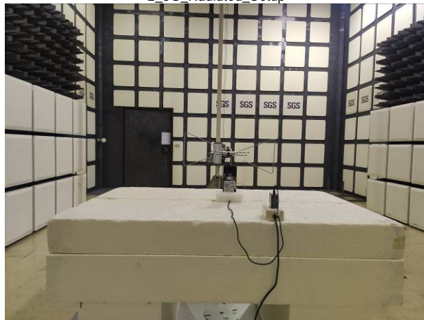
FR1_Radiated_Setup
