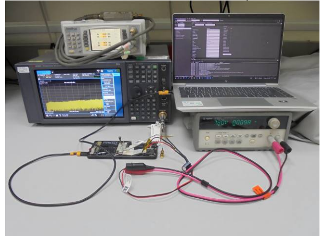
FCC_15_407_WLAN_Conducted_setup
