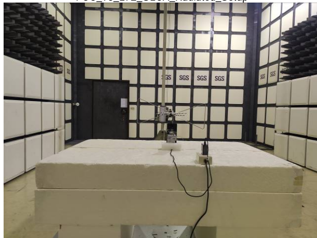
FCC_96_NR_Radiated_Setup
