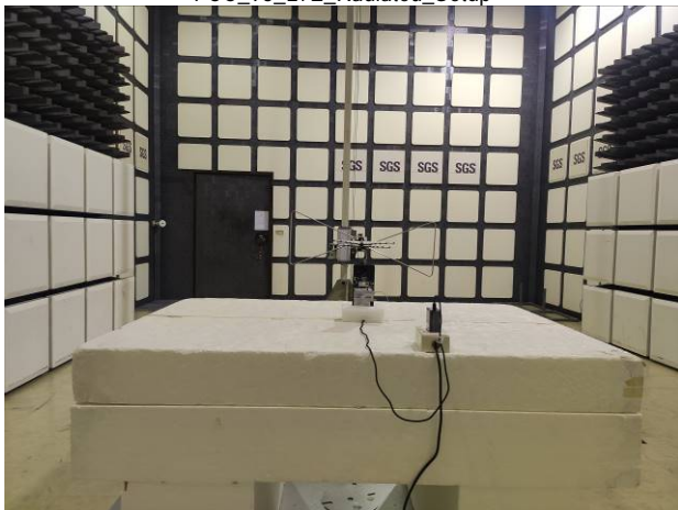
FCC_96_LTE_ULCA_Radiated_Setup
