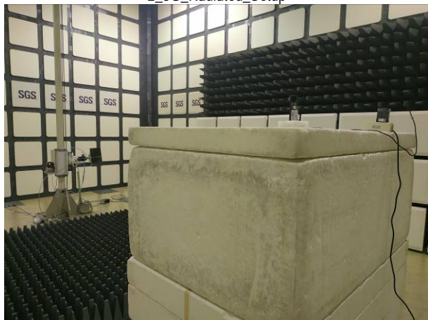
2_3G_Radiated_Setup
