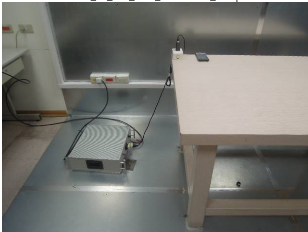
FCC_15_225_NFC_Conduction_Setup
