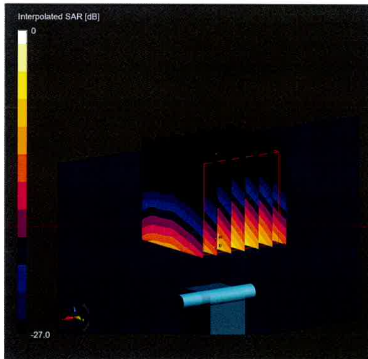
0 dB = 32.1 W/Kg
