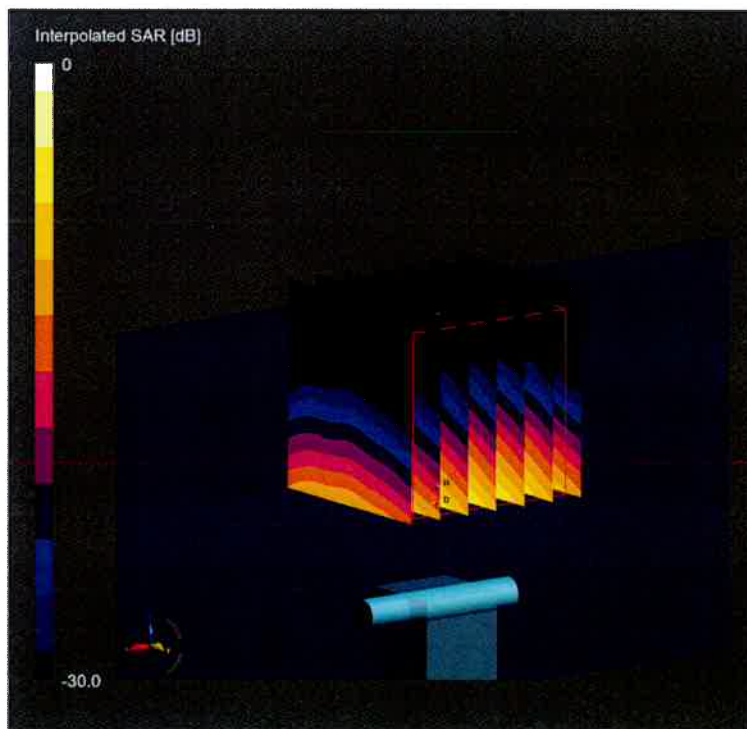
0 dB = 36.5 W/Kg
