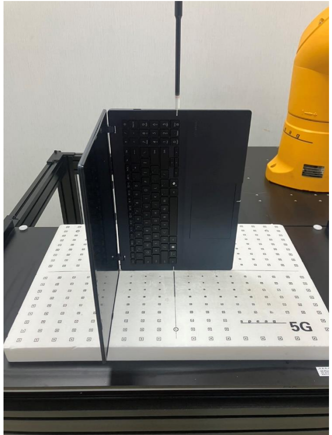
Testing Setup for Power Density, Right Edge of laptop at 2 mm
