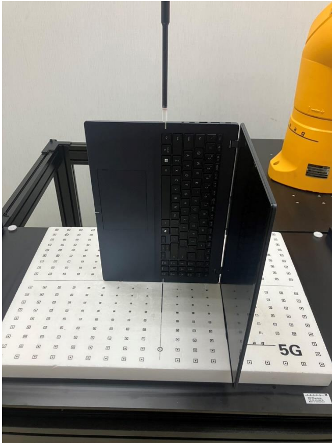
Testing Setup for Power Density, Left Edge of laptop at 2 mm
