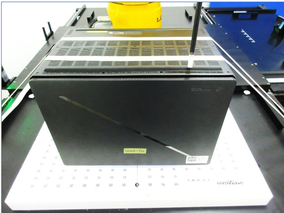
Setup for Power Density Testing (Bottom Surface of Base at 2 mm)
