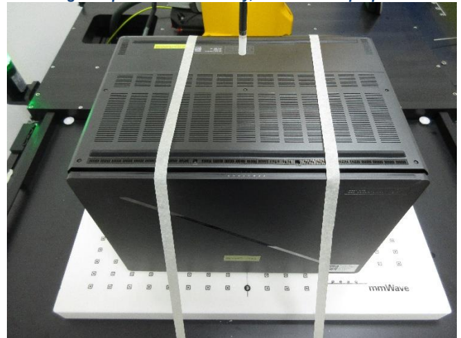
Testing Setup for Power Density, Bottom of Laptop at 2 mm
