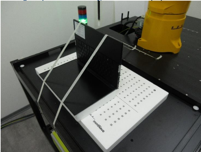
Testing Setup for Power Density, Front Side of Laptop at 0 mm-01
