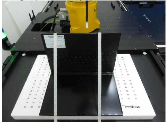
Testing Setup for Power Density, Front Side of Laptop at 0 mm-02
