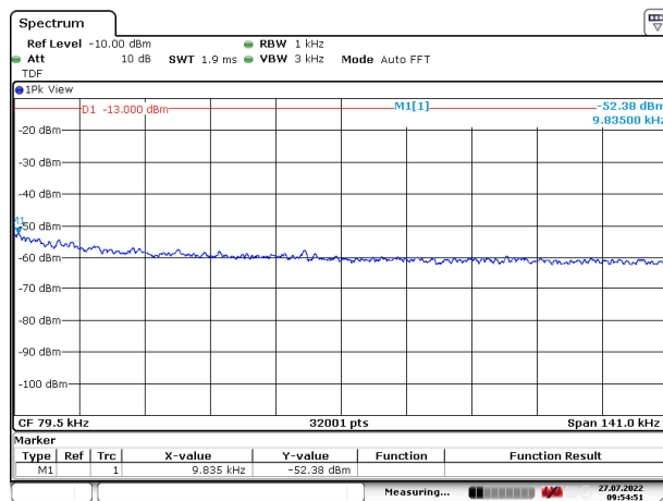
Figure 254: 9 – 150 kHz
