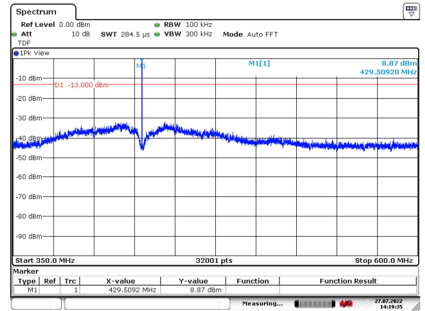
Figure 227: 350 – 600 MHz
