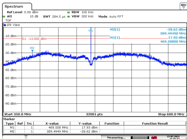
Figure 239: 350 – 600 MHz
