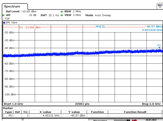
Figure 241: 1000 – 5000 MHz
