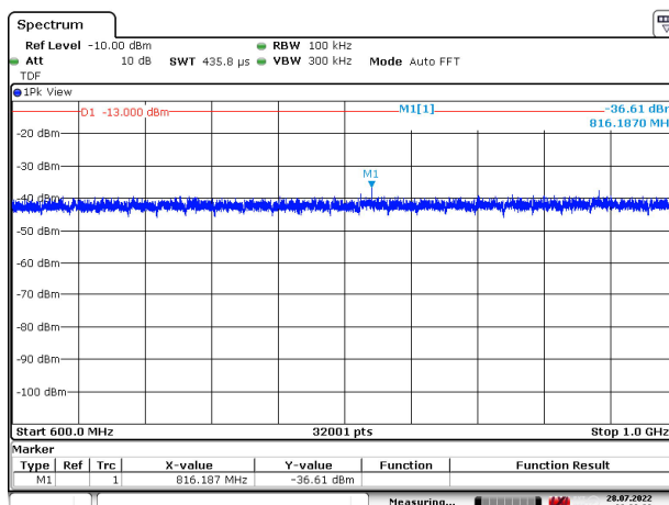
Figure 258: 600 – 1000 MHz
