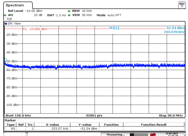
Figure 255: 150 kHz – 30 MHz
