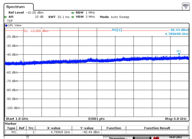
Figure 259: 1000 – 5000 MHz
