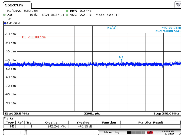
Figure 226: 30 – 350 MHz
