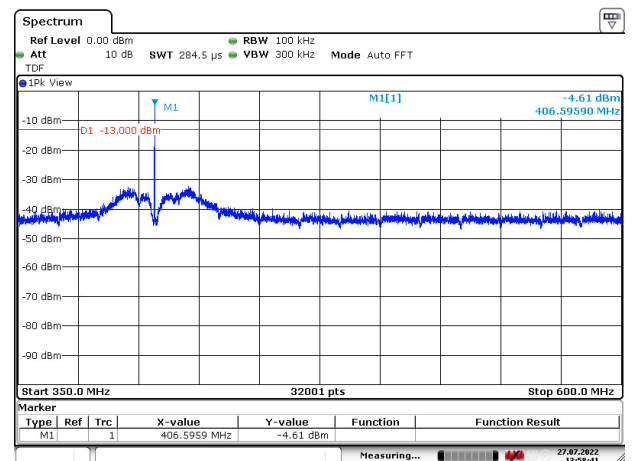
Figure 197: 350 – 600 MHz
