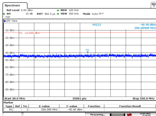
Figure 196: 30 – 350 MHz
