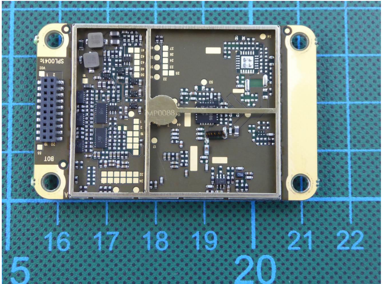
170226_31.jpg: EUT without shielding – bottom view
