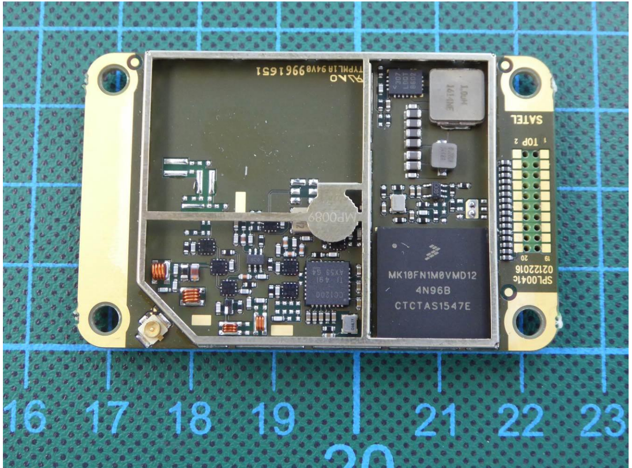
170226_32.jpg: EUT without shielding – top view
