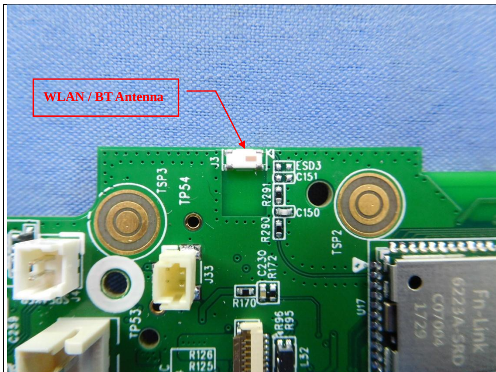
WLAN / Bluetooth Antenna
