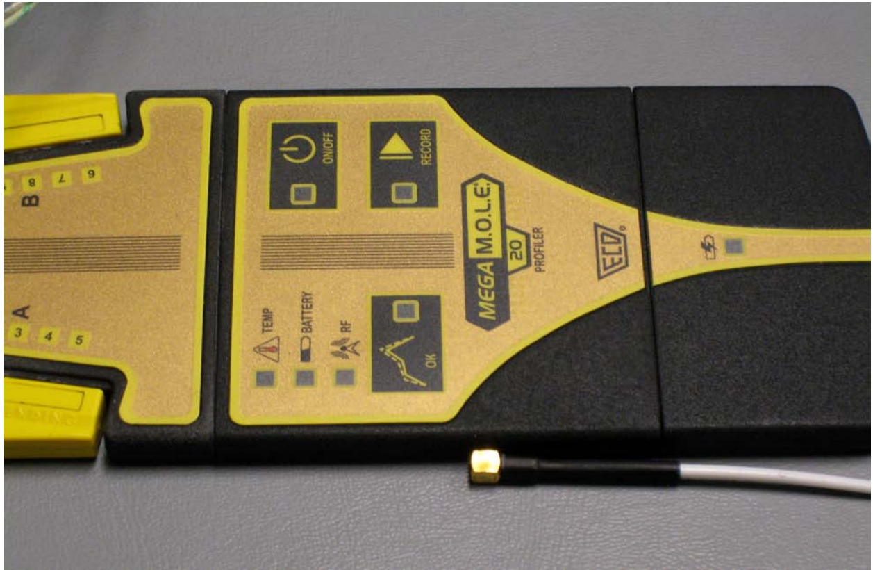
MOLE antenna connection
