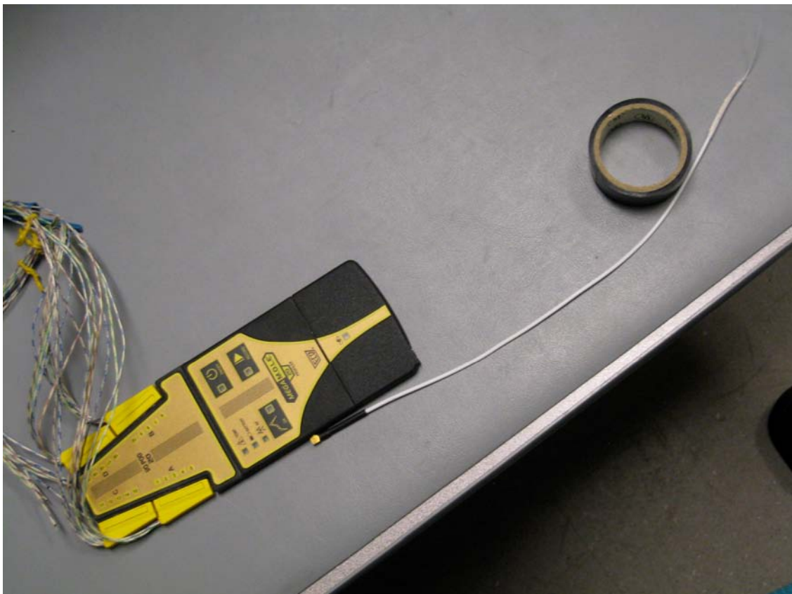
MOLE with antenna attached
