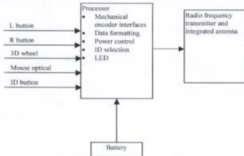
Figure 2. Mouse Unit Block Diagram
