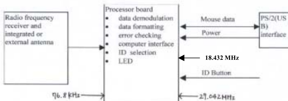
Figure 3. Receiver Block Diagram
