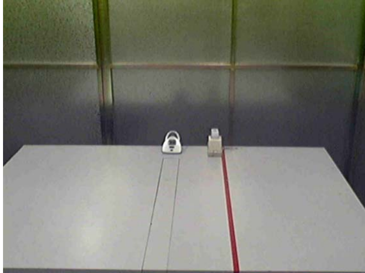
Conducted Emission
