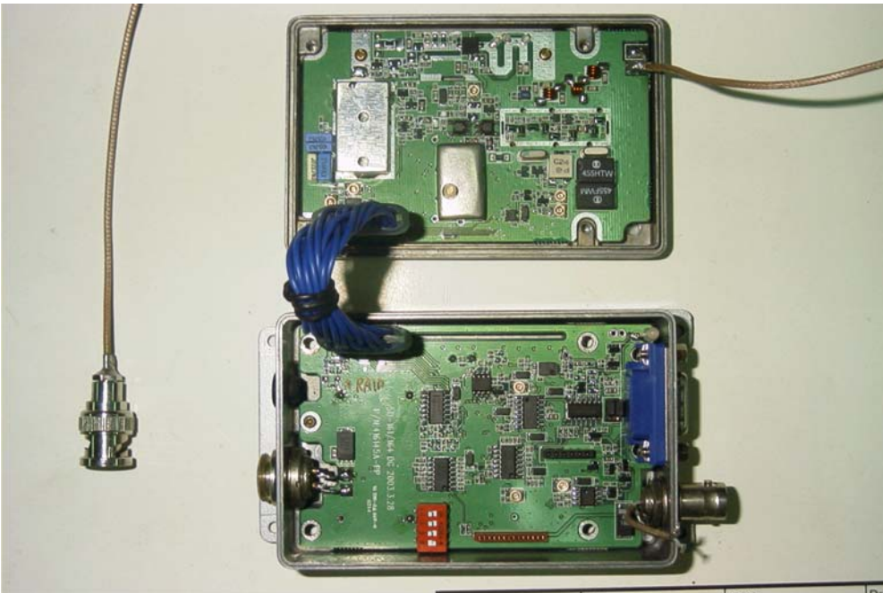
Figure 2.3. Connecting RF board to Digital board
