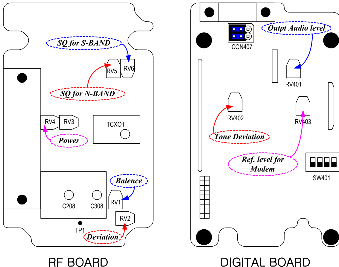
Figure 1.1. Alignment points of SD-164
