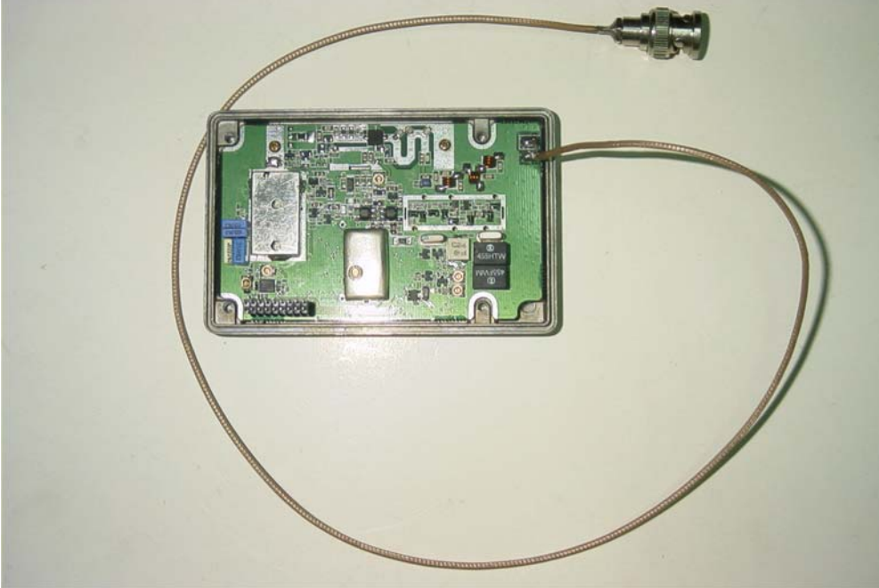
Figure 2.2. Soldering RF test cable to RF board
