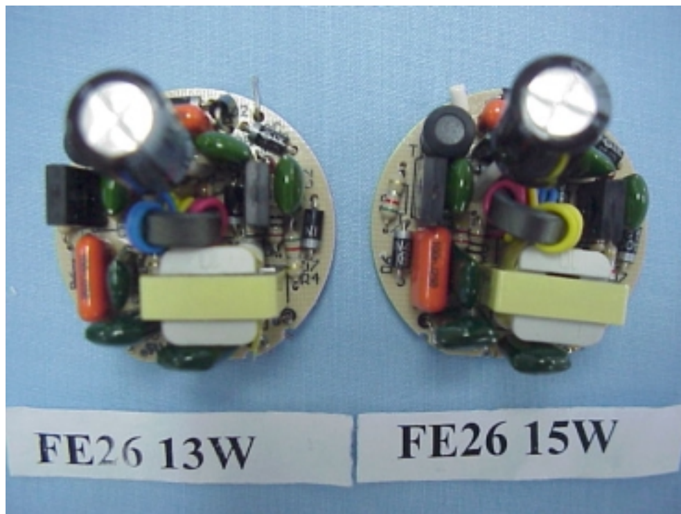
FIGURE 9 ENERGY SAVING LAMP (M/N: FE26 13W, FE26 15W) SOLDERED SIDE
