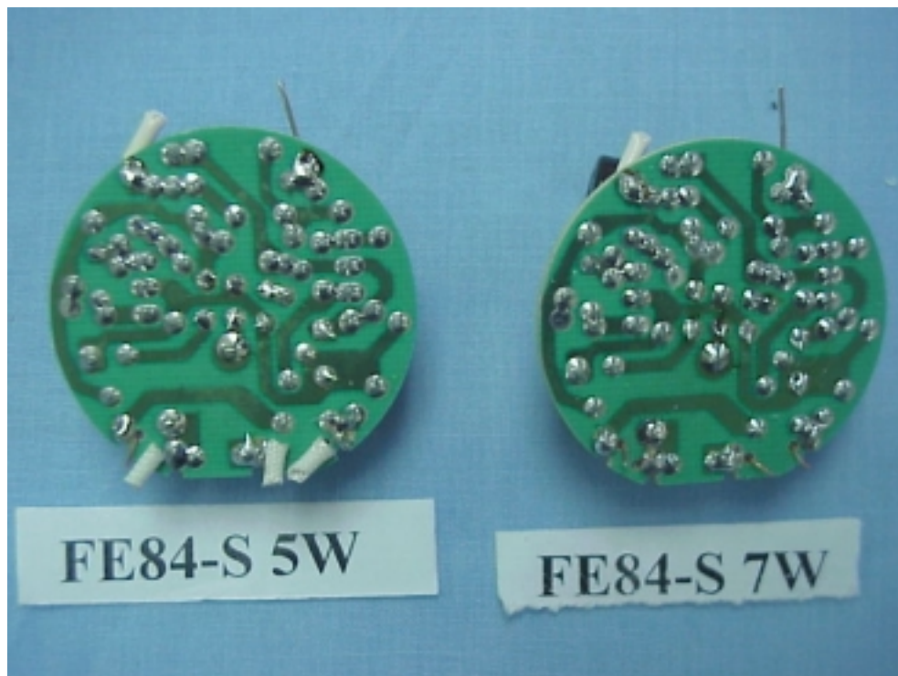
Figure 12 Energy Saving Lamp (M/N: FE84-S 5W, FE84-S 7W) SOLDERED SIDE
