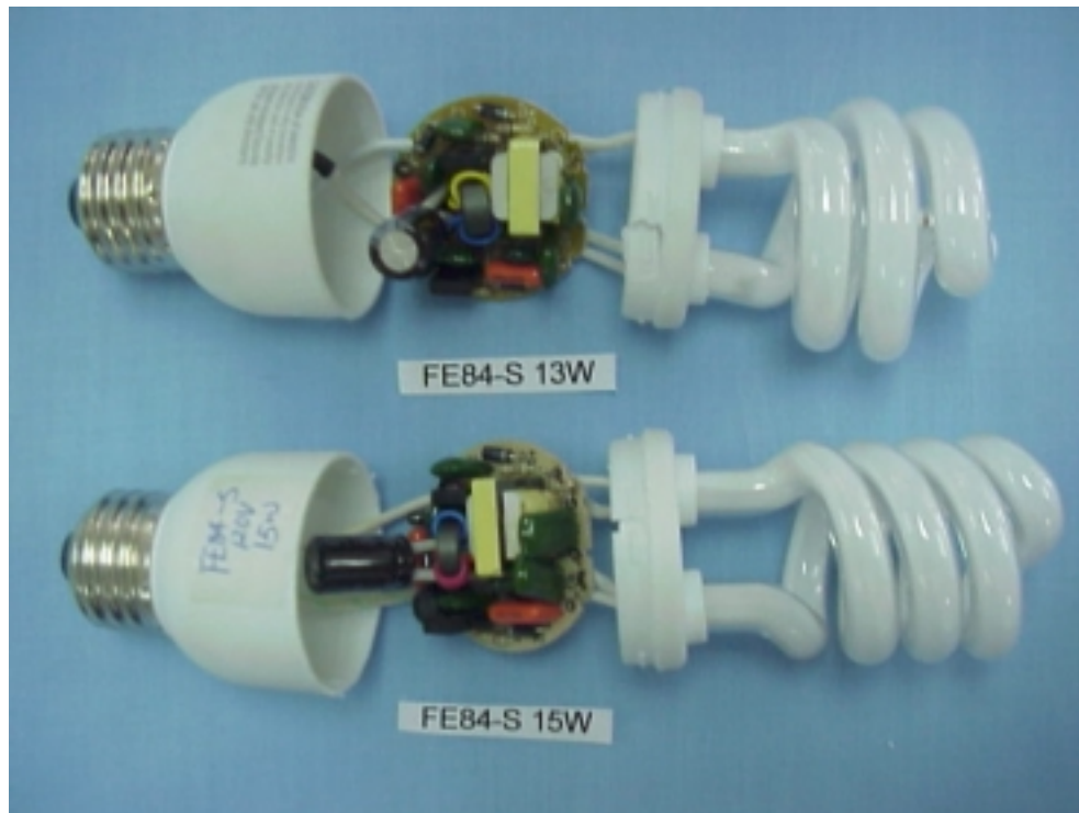
Figure 16 Energy Saving Lamp (M/N: FE84-S 13W, FE84-S 15W) GENERAL APPEARANCE
