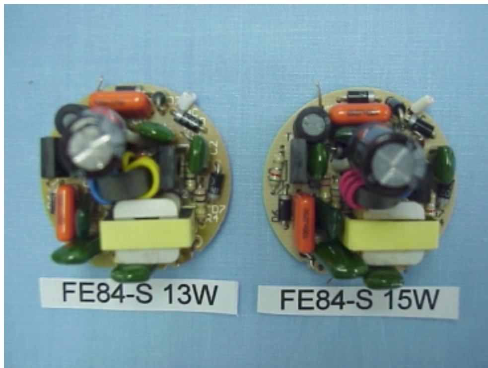
Figure 18 Energy Saving Lamp (M/N: FE84-S 13W, FE84-S 15W) SOLDERED SIDE
