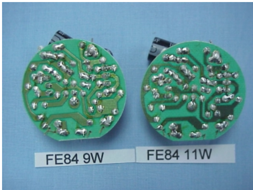
Figure 24 Energy Saving Lamp(M/N: FE84 9W, FE84 11W) SOLDERED SIDE
