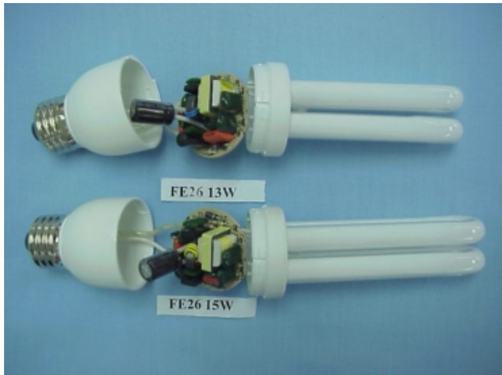
Figure 7 Energy Saving Lamp (M/N: FE26 13W, FE26 15W) Cover Removed
