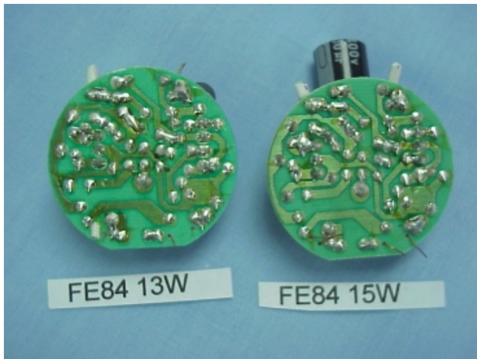
Figure 27 Energy Saving Lamp(M/N: FE84 13W, FE84 15W) SOLDERED SIDE
