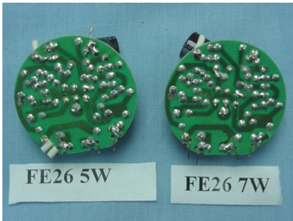
Figure 3 Energy Saving Lamp (M/N: FE26 5W, FE26 7W) SOLDERED SIDE
