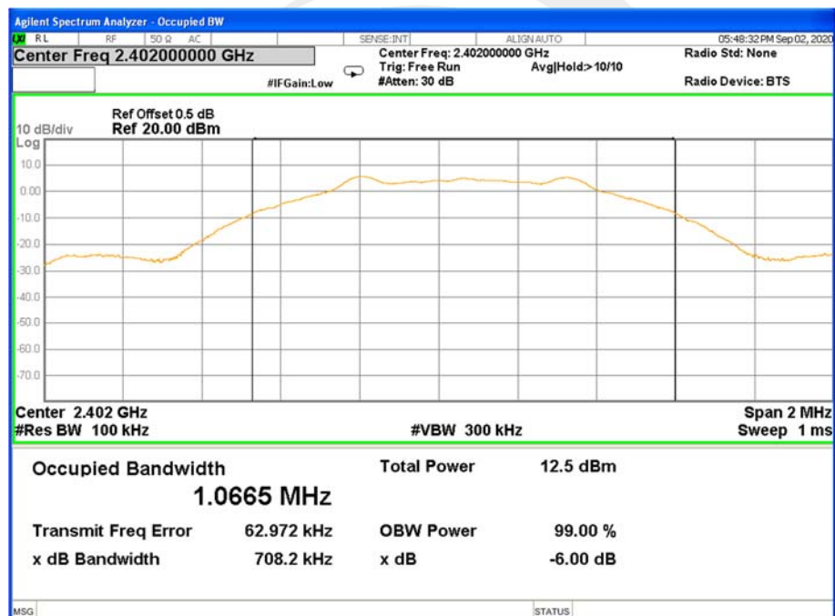
6dB Bandwidth TX CH 00
