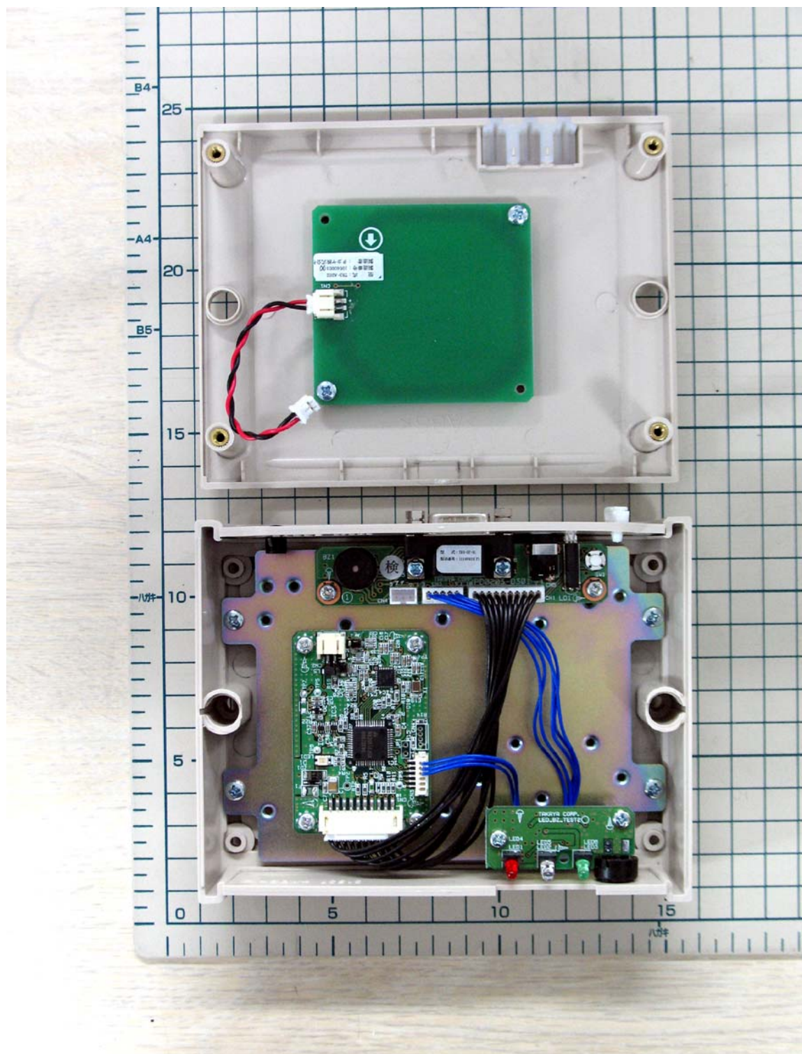
TR3XM-SD01 in Case
