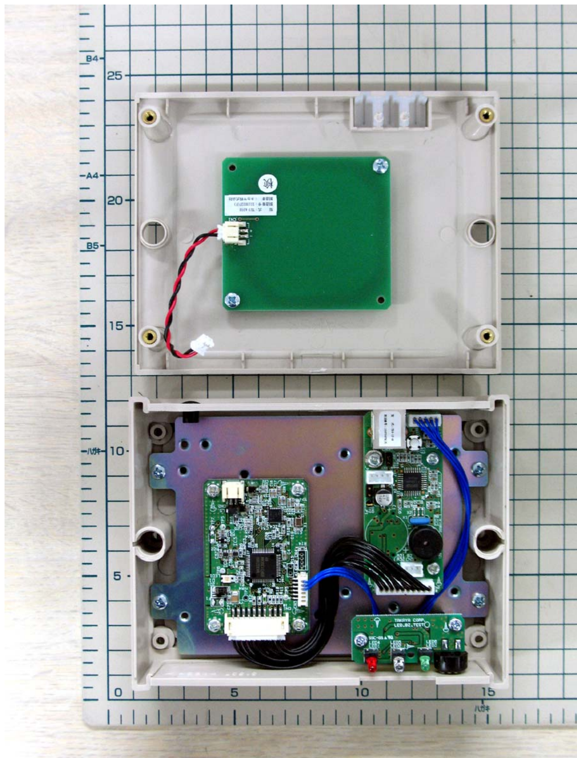
TR3XM-SU01 in Case
