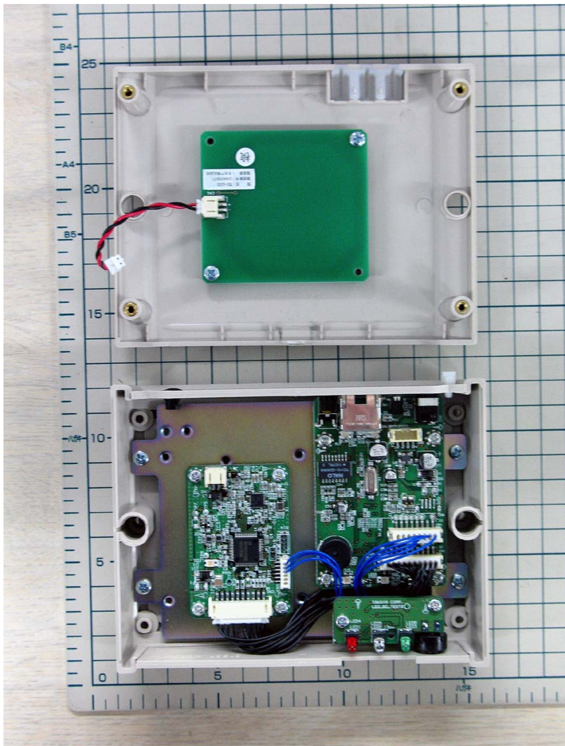
TR3XM-SN01 in Case
