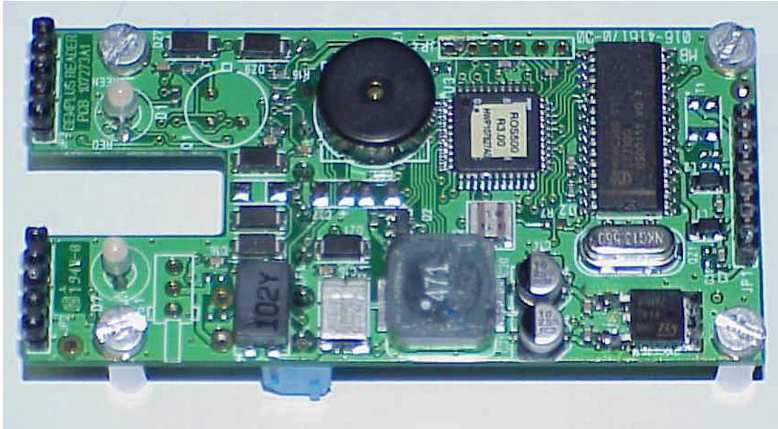
3 – Upper board, component side
