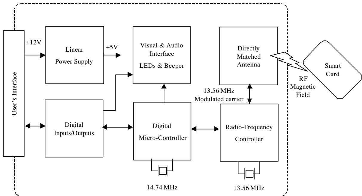
GemEasyLink/Access 3xx Block Diagram
