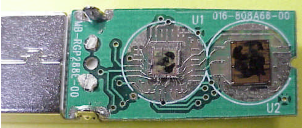
Internal board, fences removed
