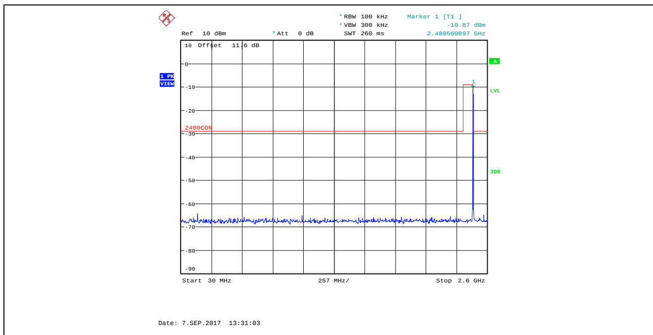
Plot 5.4.4.2.11. Conducted Spurious Emissions in Non-Restricted Frequency Bands, Low Power 2480 MHz, QPSK Modulation, 30 MHz – 2.6 GHz, Peak Detector
