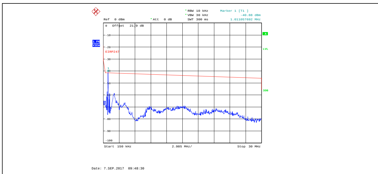
Plot 5.4.4.3.2. Conducted Spurious Emissions in Restricted Frequency Bands, High Power 2405 MHz, QPSK Modulation, 150 kHz - 30 MHz, Peak Detector Marker 1 is Outside of the Restricted Bands
