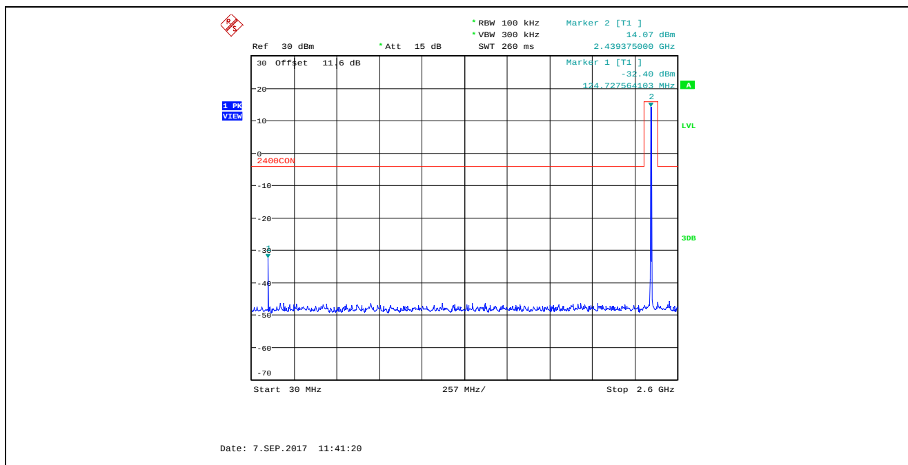
Plot 5.4.4.2.3. Conducted Spurious Emissions in Non-Restricted Frequency Bands, High Power 2440 MHz, QPSK Modulation, 30 MHz – 2.6 GHz, Peak Detector
