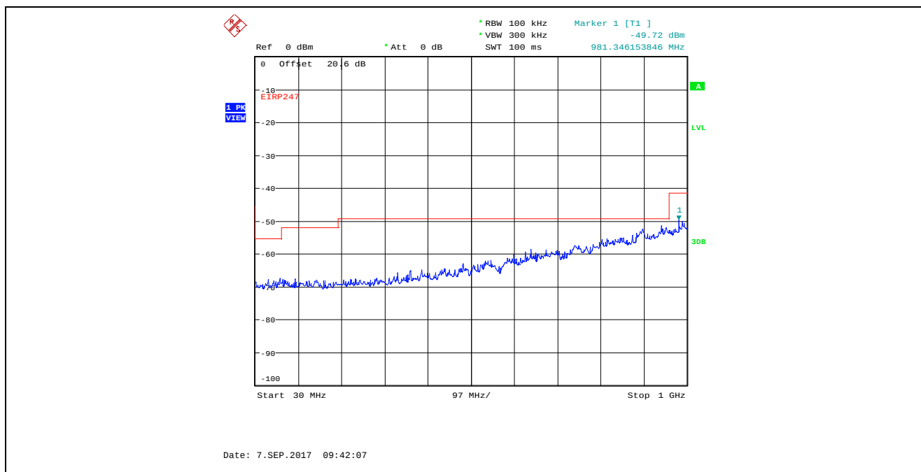
Plot 5.4.4.3.15. Conducted Spurious Emissions in Restricted Frequency Bands, High Power 2480 MHz, QPSK Modulation, 30 MHz - 1 GHz, Peak Detector
