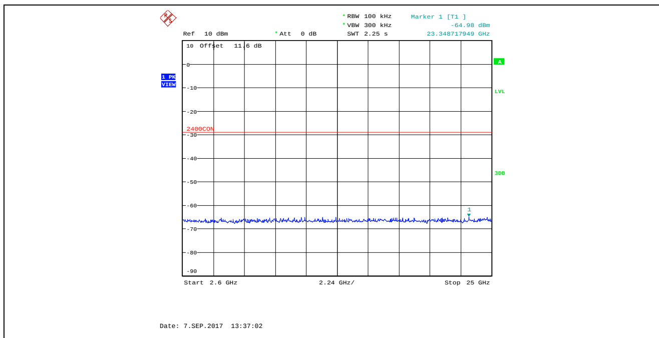
Plot 5.4.4.2.12. Conducted Spurious Emissions in Non-Restricted Frequency Bands, Low Power 2480 MHz, QPSK Modulation, 2.6 GHz – 25 GHz, Peak Detector
