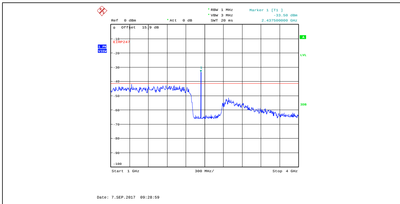
Plot 5.4.4.3.10. Conducted Spurious Emissions in Restricted Frequency Bands, High Power 2440 MHz, QPSK Modulation, 1 GHz - 4 GHz, Peak Detector Marker 1 is the Fundamental Frequency
