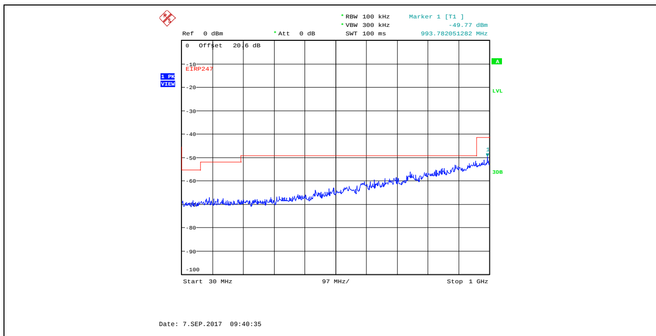
Plot 5.4.4.3.9. Conducted Spurious Emissions in Restricted Frequency Bands, High Power 2440 MHz, QPSK Modulation, 30 MHz - 1 GHz, Peak Detector
