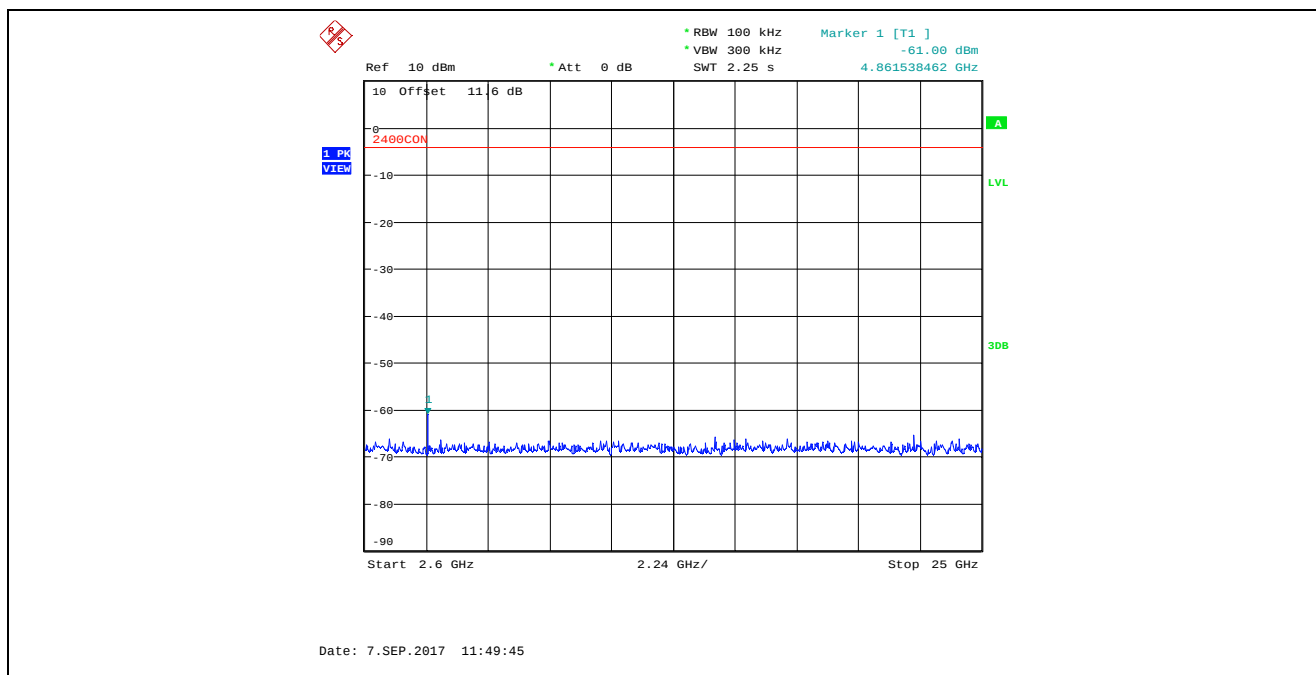
Plot 5.4.4.2.4. Conducted Spurious Emissions in Non-Restricted Frequency Bands, High Power 2440 MHz, QPSK Modulation, 2.6 GHz – 25 GHz, Peak Detector
