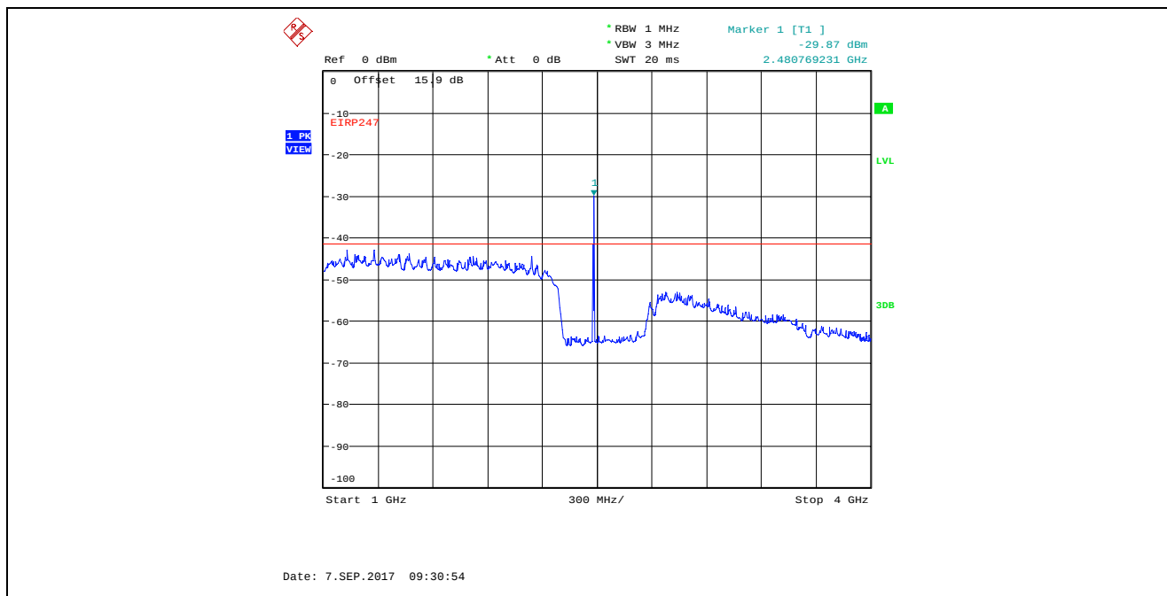
Plot 5.4.4.3.16. Conducted Spurious Emissions in Restricted Frequency Bands, High Power 2480 MHz, QPSK Modulation, 1 GHz - 4 GHz, Peak Detector Marker 1 is the Fundamental Frequency
