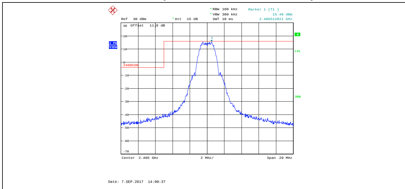
Plot 5.4.4.1.1. Band-Edge RF Conducted Emissions QPSK Modulation, High Power, Ch 11, 2405 MHz, Lower Band-edge
