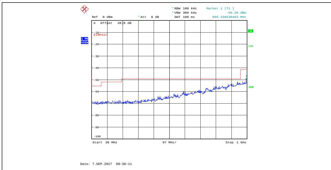
Plot 5.4.4.3.3. Conducted Spurious Emissions in Restricted Frequency Bands, High Power 2405 MHz, QPSK Modulation, 30 MHz - 1 GHz, Peak Detector
