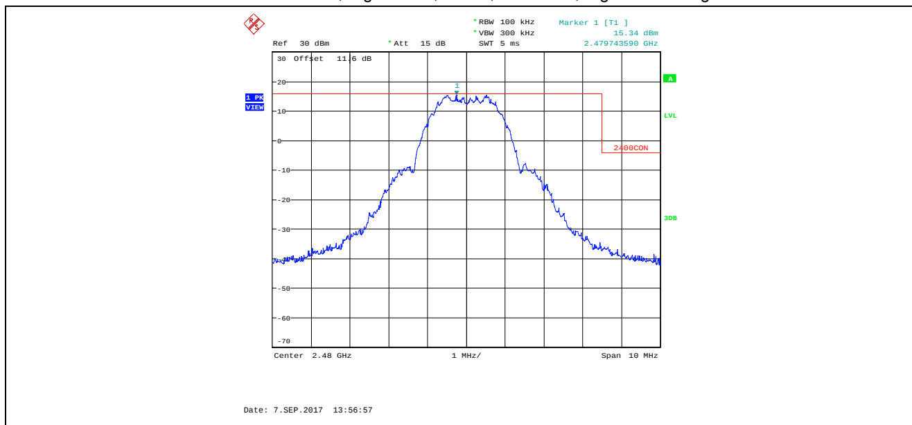
Plot 5.4.4.1.2. Band-Edge RF Conducted Emissions QPSK Modulation, High Power, CH 26, 2480 MHz, Higher Band-edge
