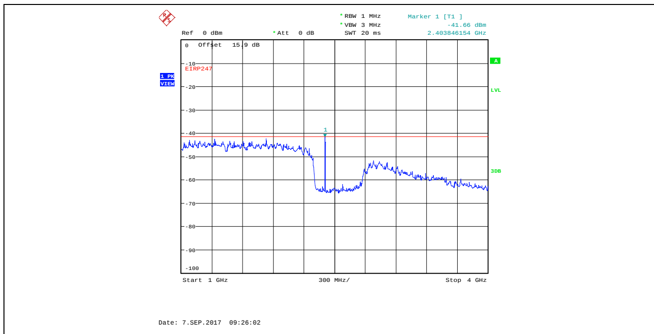
Plot 5.4.4.3.4. Conducted Spurious Emissions in Restricted Frequency Bands, High Power 2405 MHz, QPSK Modulation, 1 GHz - 4 GHz, Peak Detector Marker 1 is the Fundamental Frequency
