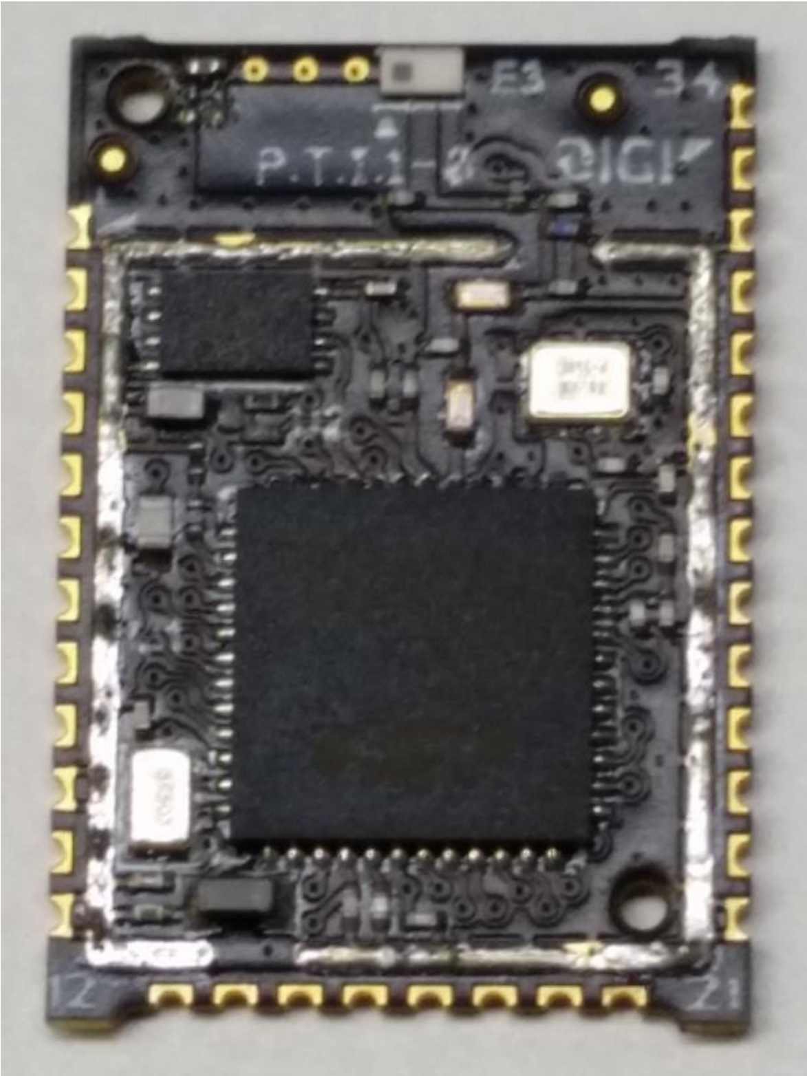
Chip Antenna Interior
