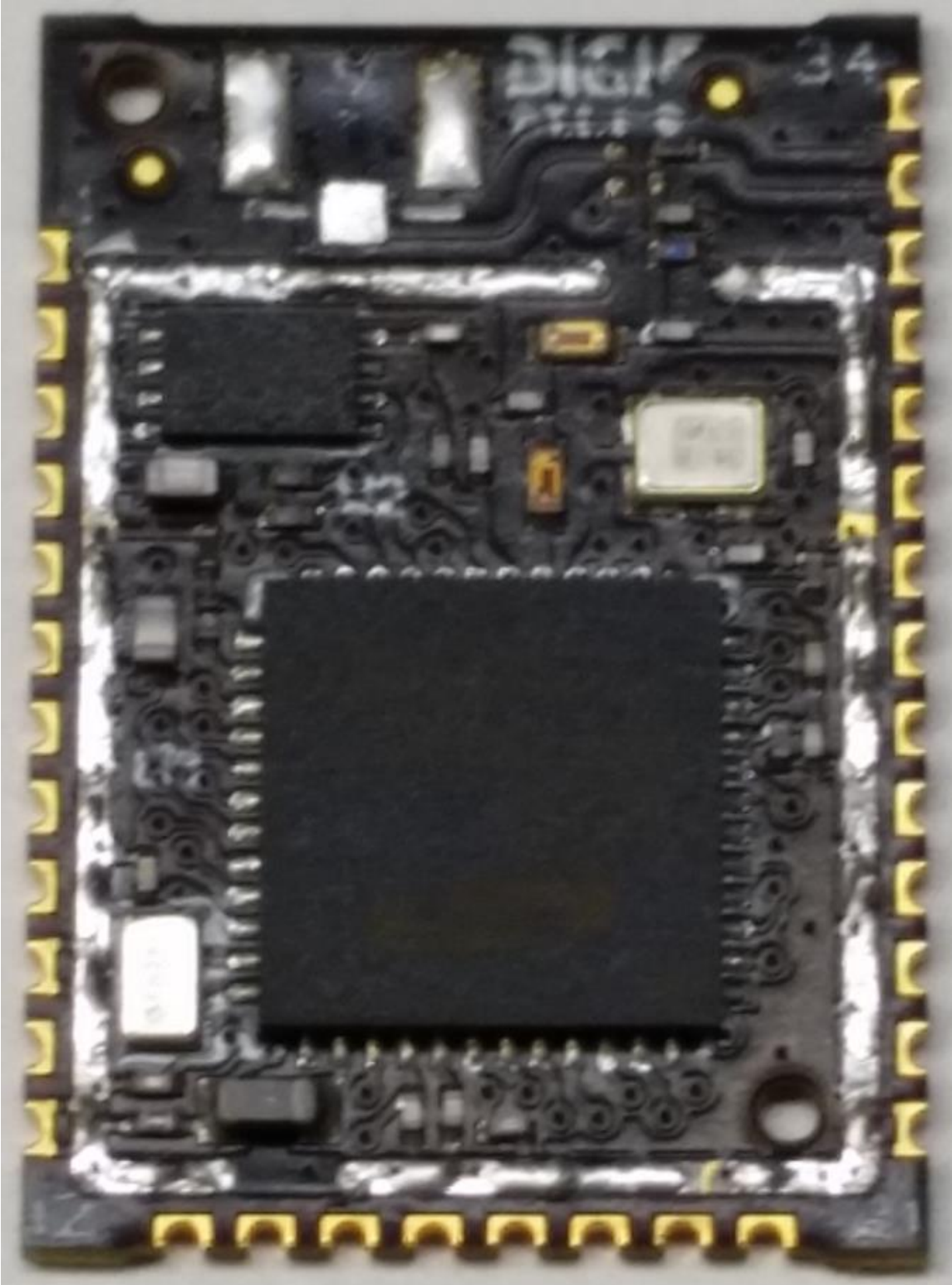
RF Pad Interior
