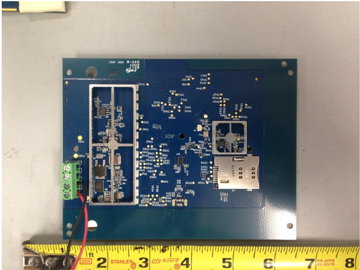
Bottom without shields
