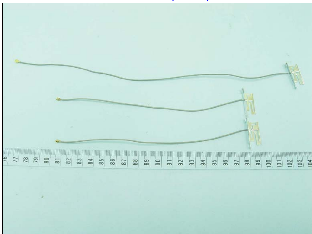
Laird antenna (4.17dBi)
