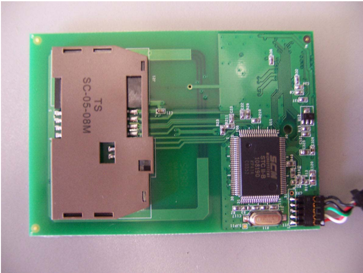
EUT PCB Top View
