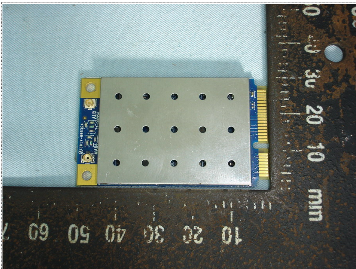
Front View of EUT-1 (WLL4080-D12)
