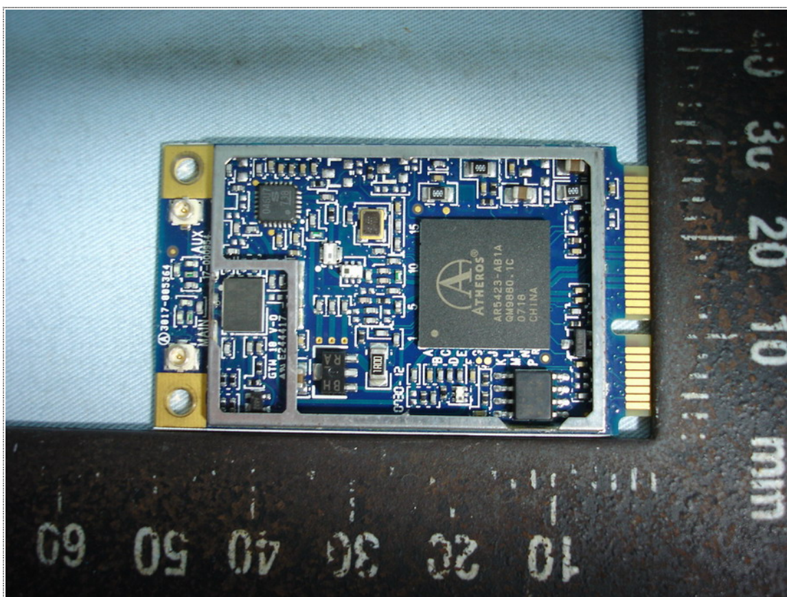
Front View of EUT-2 (WLL4080-D12)
